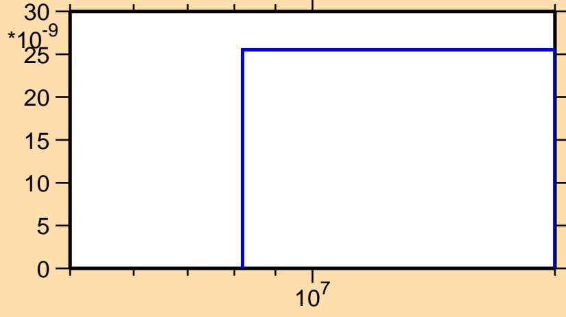
\sigma vs. E for ^{190}\text{Pt}(n,2n\alpha)
