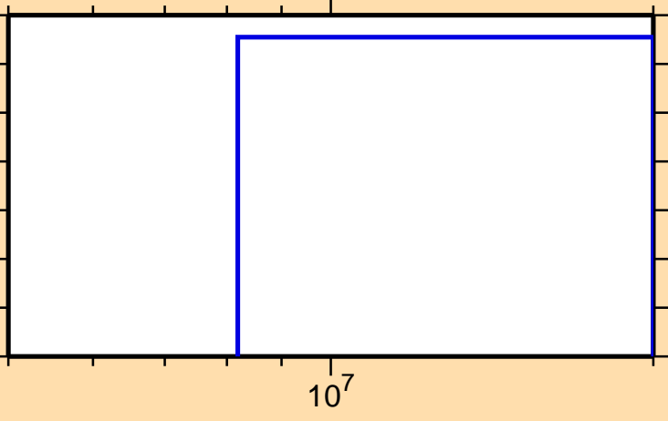
\sigma vs. E for ^{190}\text{Pt}(n,t)
