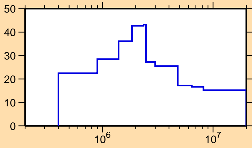
\Delta\sigma/\sigma vs. E for ^{191}\text{Pt}(n,n_1)
