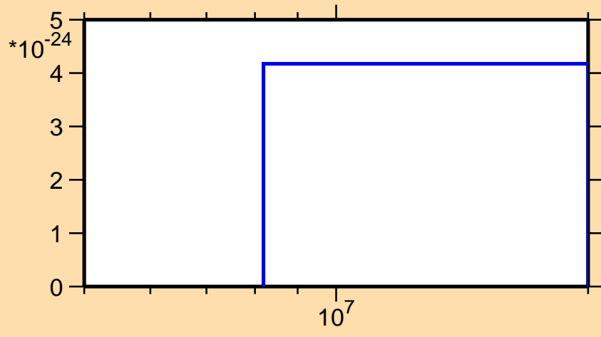
\sigma vs. E for ^{191}\text{Pt}(\text{mt } 11)
