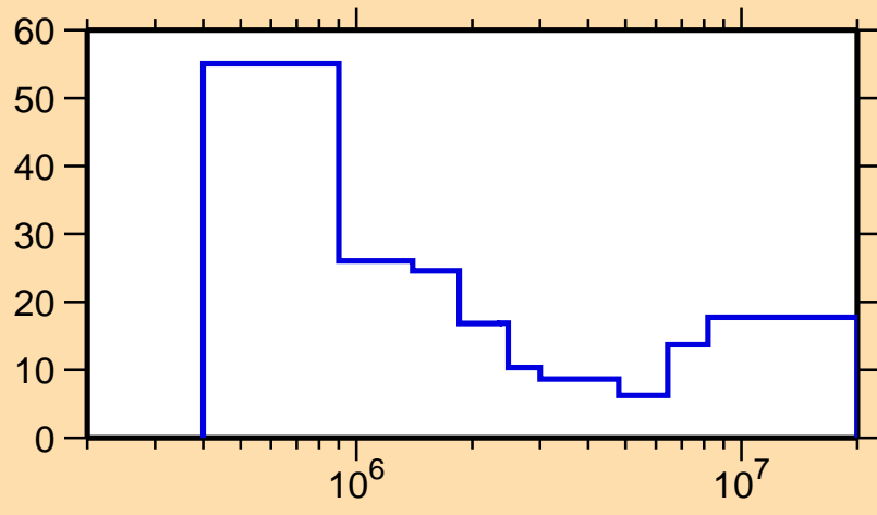
\Delta\sigma/\sigma vs. E for ^{191}\text{Pt}(n,n\text{cont.})
