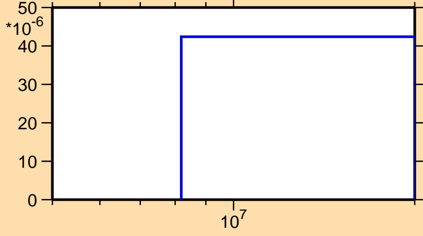
\sigma vs. E for ^{191}\text{Pt}(n,t)
