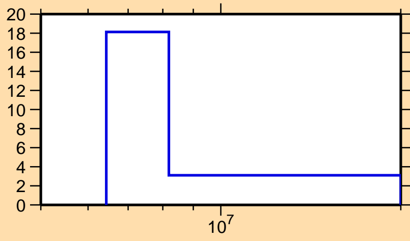
\Delta\sigma/\sigma vs. E for ^{191}\text{Pt}(n,2n)
