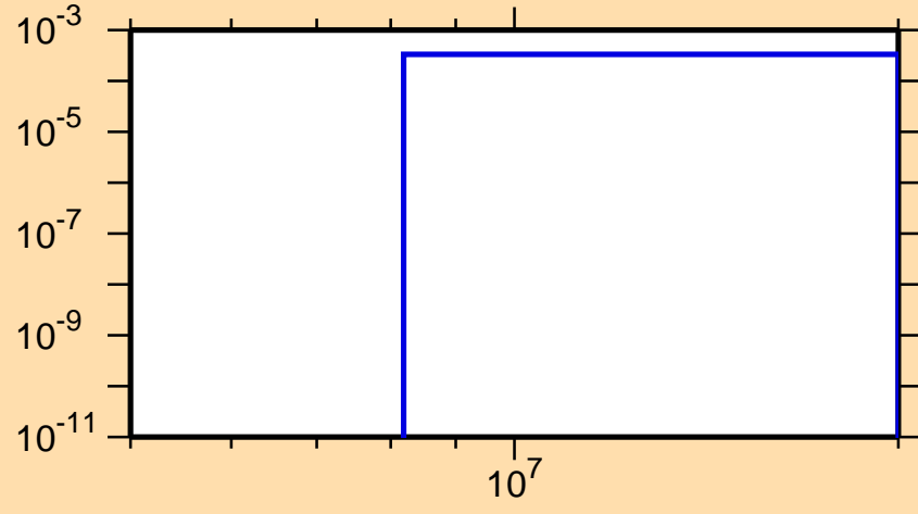
\sigma vs. E for ^{191}\text{Pt}(n,np)
