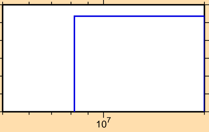
\sigma vs. E for ^{191}\text{Pt}(n,2n\alpha)
