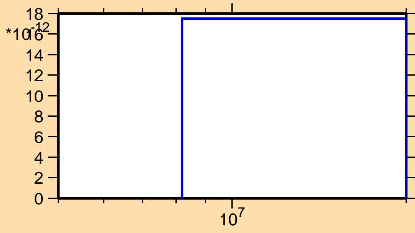
\sigma vs. E for ^{191}\text{Pt}(n,p\alpha)
