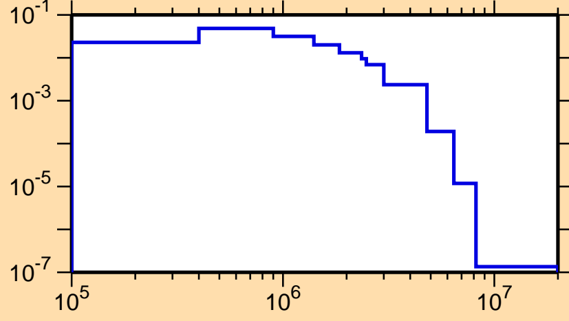
\sigma vs. E for ^{191}\text{Pt}(n,n_3)
