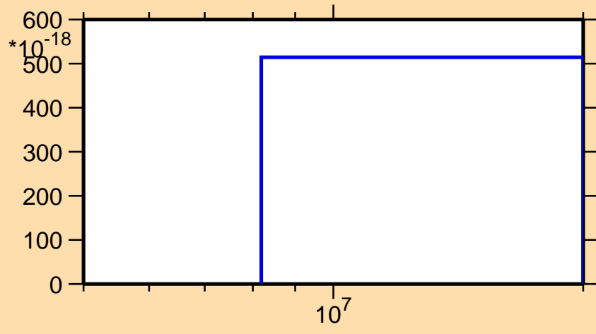
\sigma vs. E for ^{191}\text{Pt}(n,3n\alpha)
