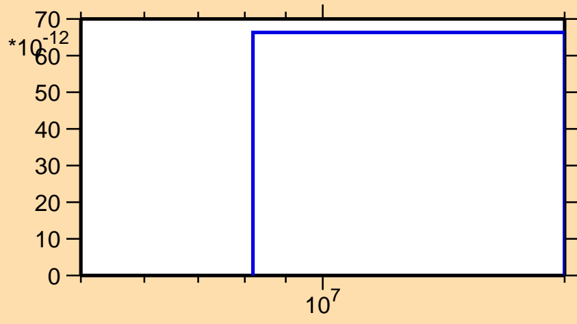
\sigma vs. E for ^{191}\text{Pt}(n,\text{He3})
