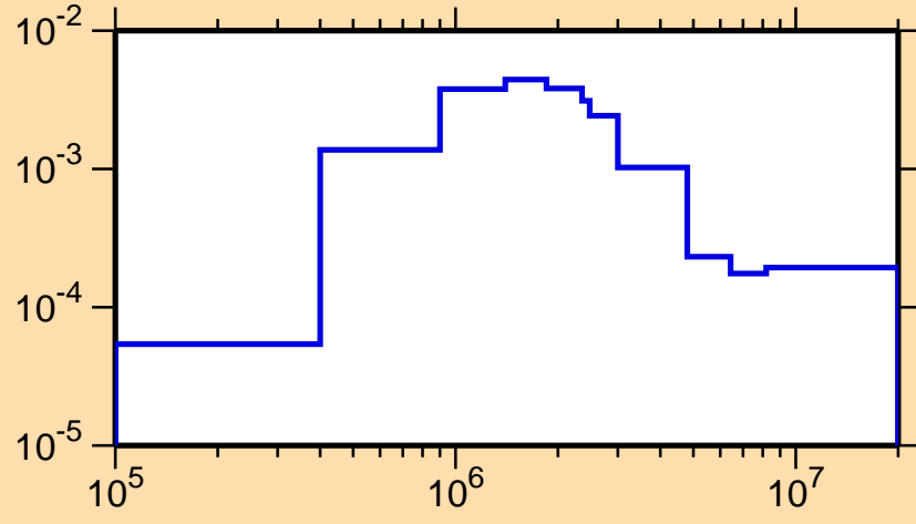
\sigma vs. E for ^{191}\text{Pt}(n,n_4)
