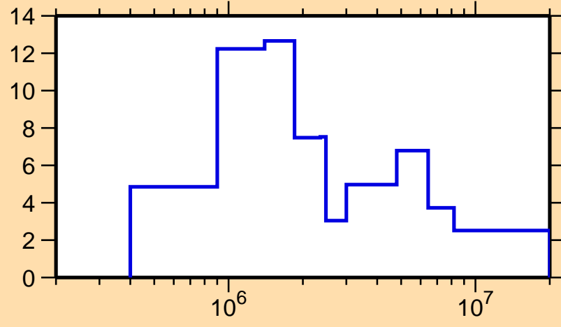
\Delta\sigma/\sigma vs. E for ^{191}\text{Pt}(n, el.)
