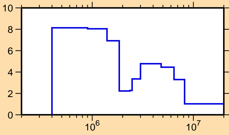
\Delta\sigma/\sigma vs. E for ^{191}\text{Pt}(n,\text{tot.})
