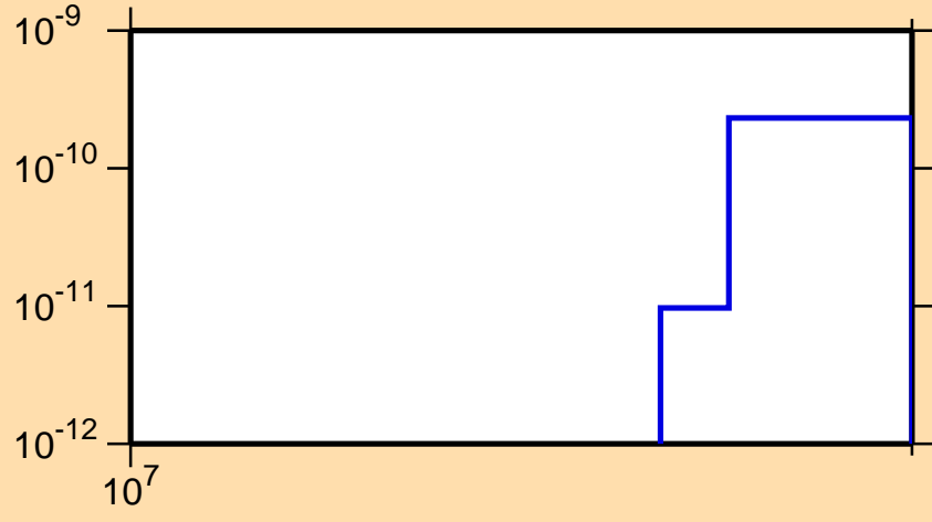
\sigma vs. E for ^{192}\text{Pt}(n,\text{He}3)
