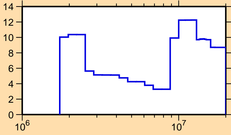
\Delta\sigma/\sigma vs. E for ^{192}\text{Pt}(n,\text{inel.})
