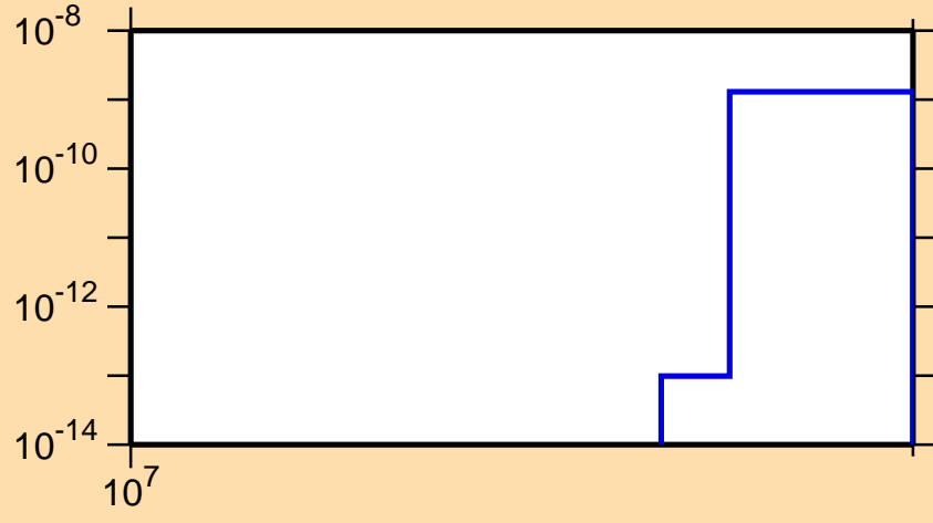
\sigma vs. E for ^{192}\text{Pt}(n,nt)
