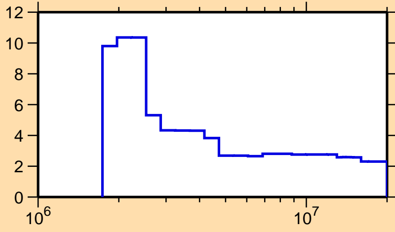
\Delta\sigma/\sigma vs. E for ^{192}\text{Pt}(n,\text{nonel.})
