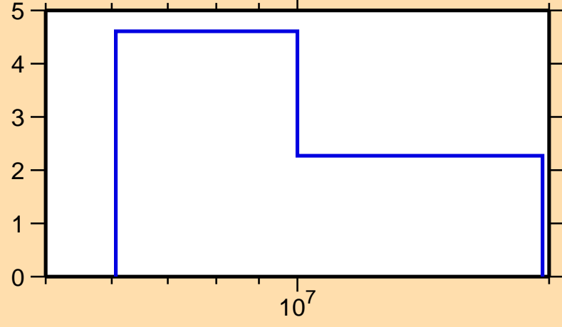
\Delta\sigma/\sigma vs. E for ^{192}\text{Pt}(n,\text{el.})
