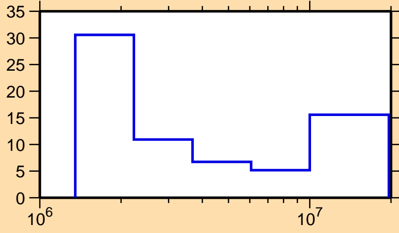
\Delta\sigma/\sigma vs. E for ^{192}\text{Pt}(n,n\text{cont.})
