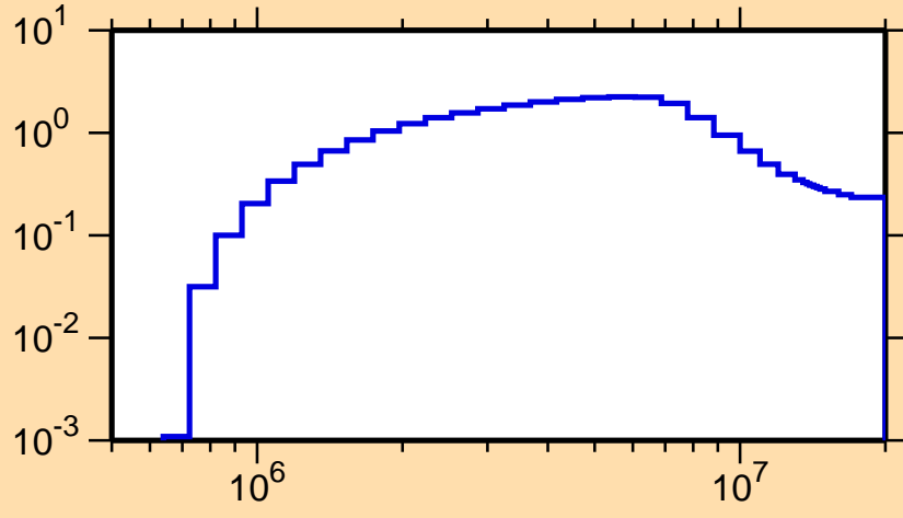
\sigma vs. E for ^{193}\text{Pt}(n,n\text{cont.})
