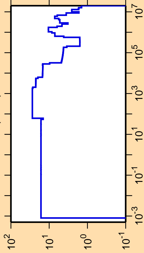
\Delta\sigma/\sigma vs. E for ^{193}\text{Pt}(n,\text{el.})
