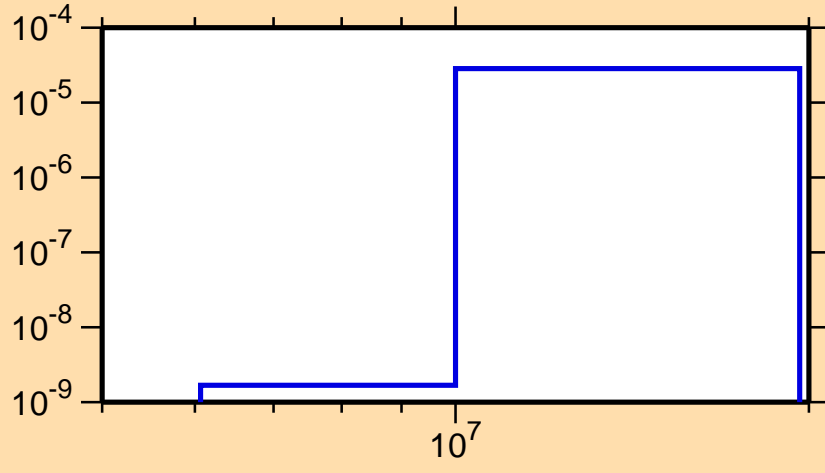
\sigma vs. E for ^{193}\text{Pt}(n,n\alpha)
