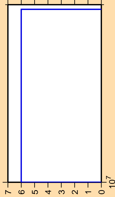
\Delta\sigma/\sigma vs. E for ^{193}\text{Pt}(n,3n)
