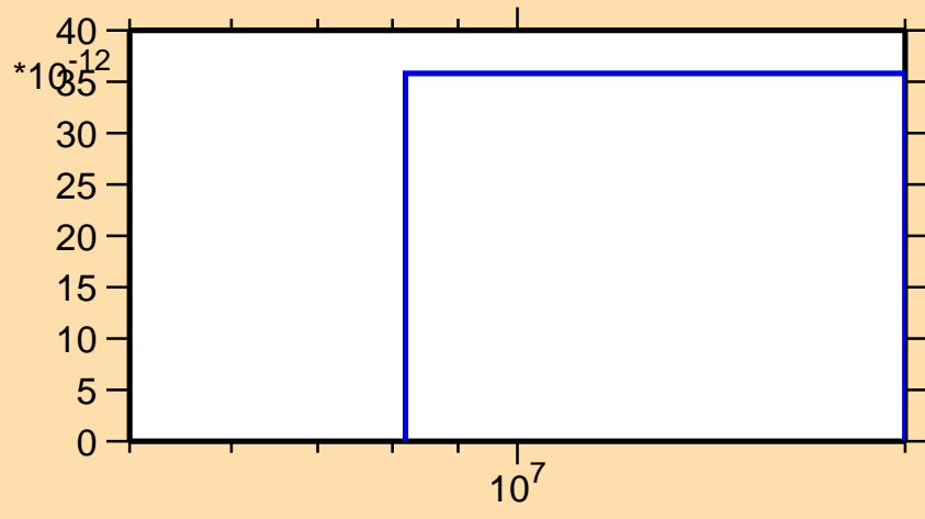
\sigma vs. E for ^{193}\text{Pt}(n,nt)
