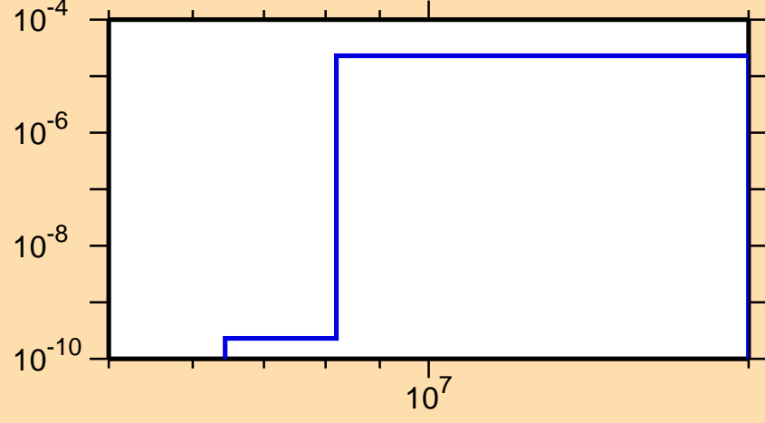
\sigma vs. E for ^{193}\text{Pt}(n,n\alpha)
