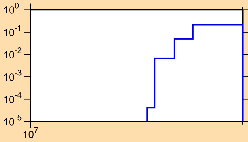
\sigma vs. E for ^{194}\text{Pt}(n,3n)
