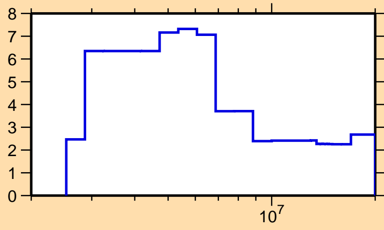
\Delta\sigma/\sigma vs. E for ^{194}\text{Pt}(n,el.)
