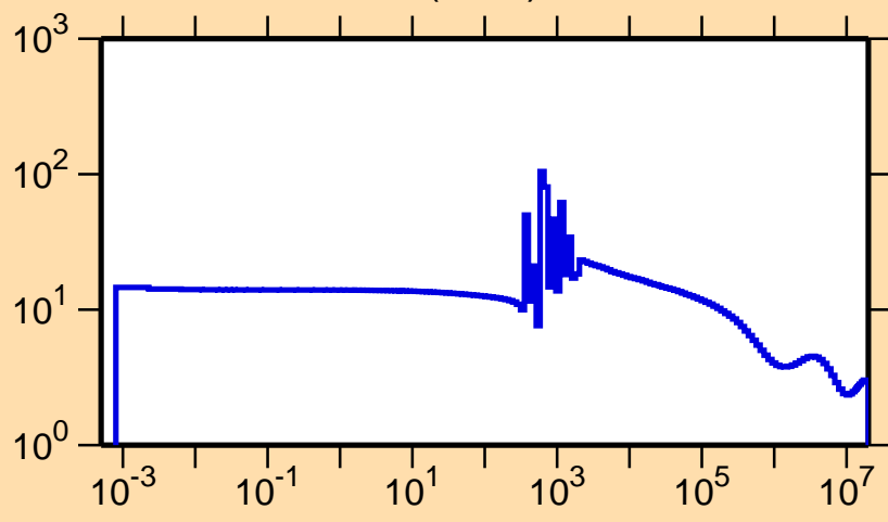
\sigma vs. E for ^{194}\text{Pt}(n,\text{el.})
