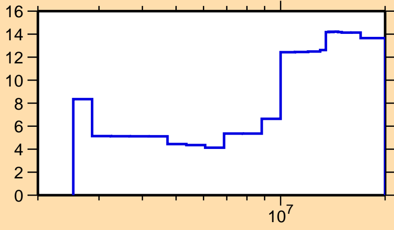
\Delta\sigma/\sigma vs. E for ^{194}\text{Pt}(n,ncont.)
