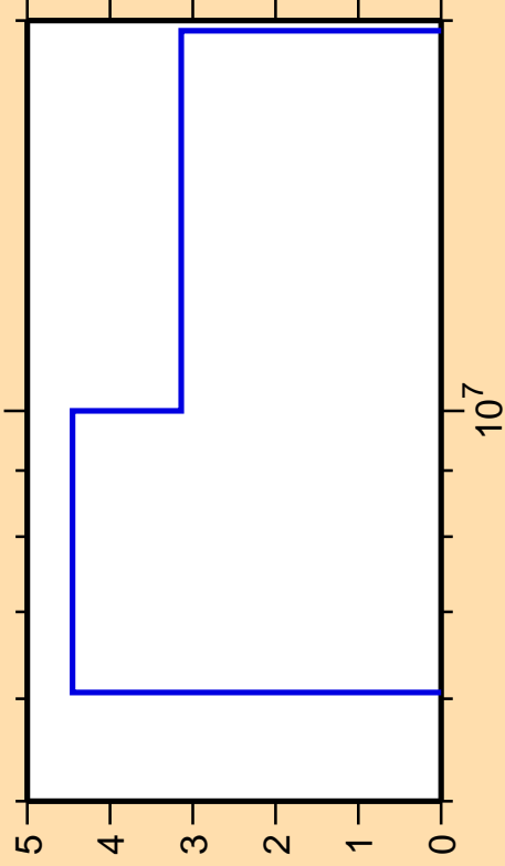
\Delta\sigma/\sigma vs. E for ^{194}\text{Pt}(n,2n)
