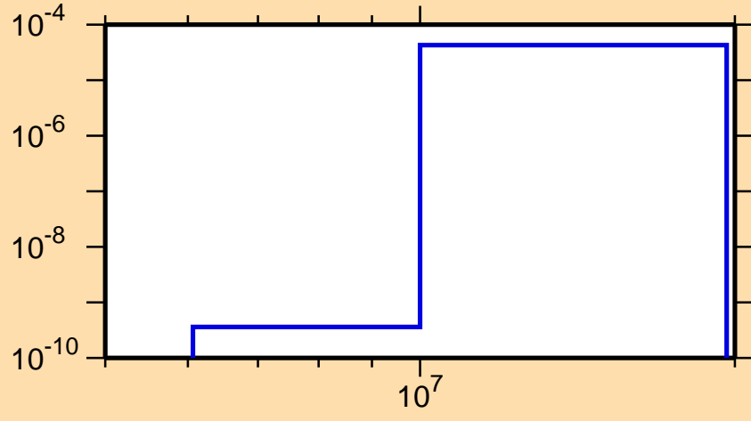
\sigma vs. E for ^{195}\text{Pt}(n,n\alpha)
