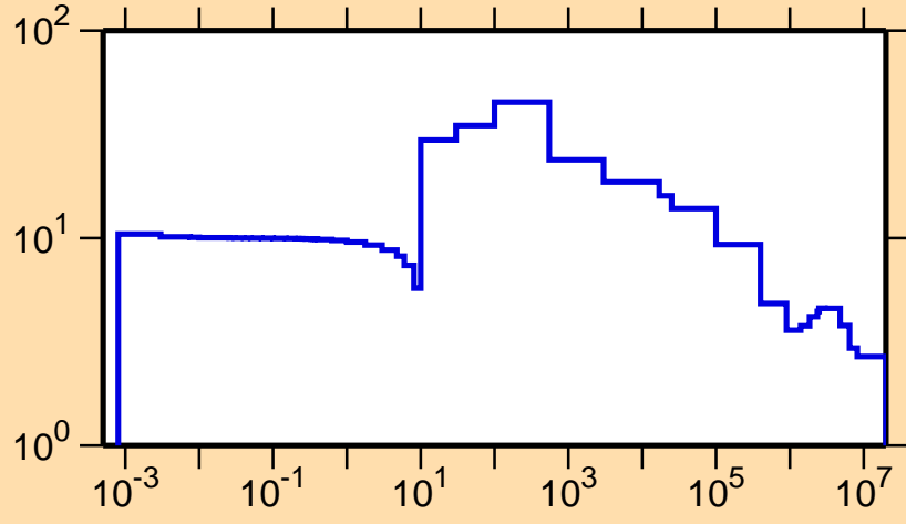
\sigma vs. E for ^{195}\text{Pt}(n,\text{el.})
