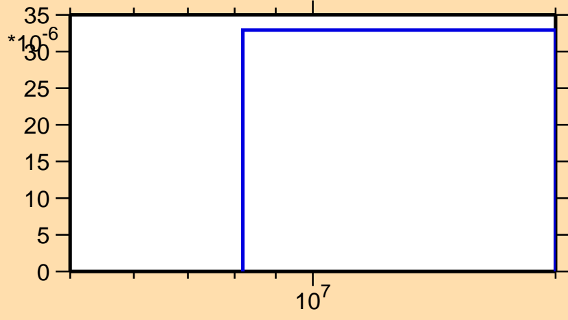
\sigma vs. E for ^{195}\text{Pt}(n,t)
