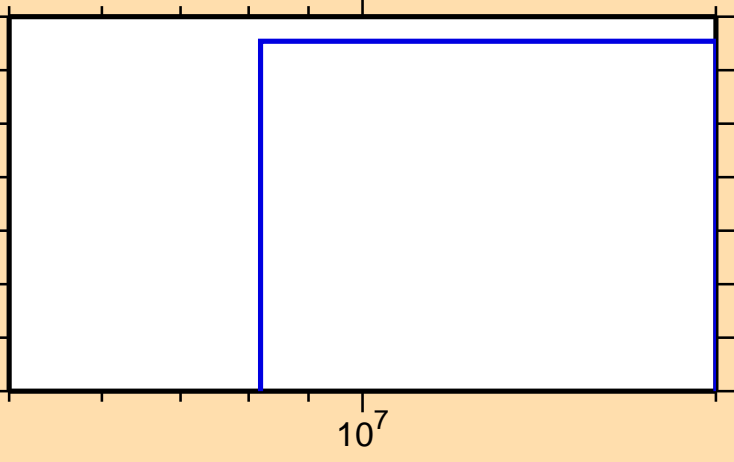
\sigma vs. E for ^{195}\text{Pt}(n,\text{nd})
