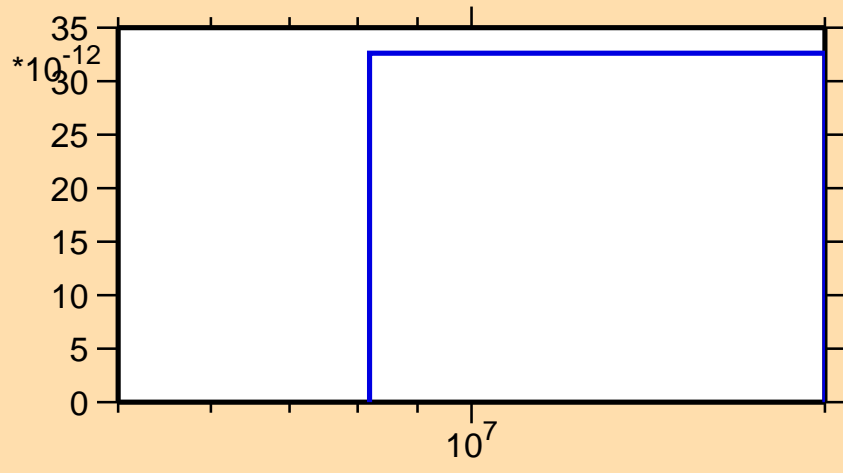
\sigma vs. E for ^{195}\text{Pt}(n,nt)
