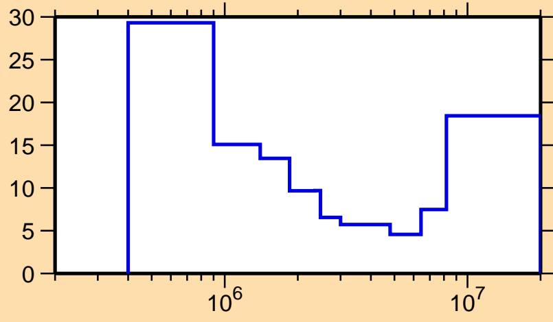
\Delta\sigma/\sigma vs. E for ^{195}\text{Pt}(n,n\text{cont.})
