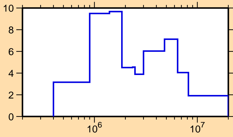
\Delta\sigma/\sigma vs. E for ^{195}\text{Pt}(n, el.)
