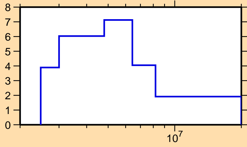
\Delta\sigma/\sigma vs. E for ^{195}\text{Pt}(n,\text{el.})
