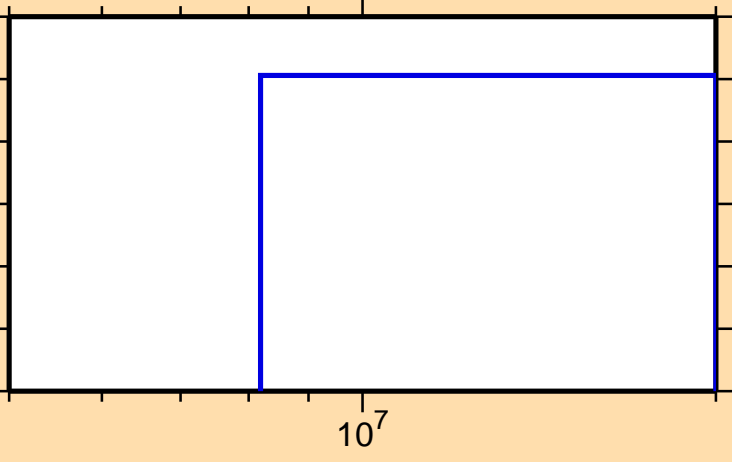
\sigma vs. E for ^{195}\text{Pt}(n,d)
