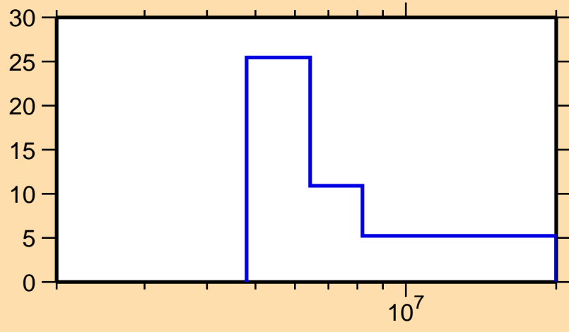
\Delta\sigma/\sigma vs. E for ^{195}\text{Pt}(n,2n)
