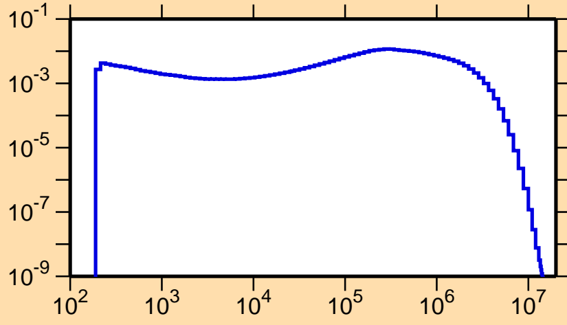
\sigma vs. E for ^{195}\text{Pt}(n,n_3)
