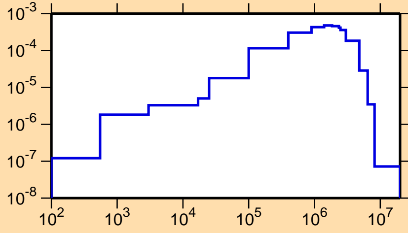
\sigma vs. E for ^{195}\text{Pt}(n,n_1)
