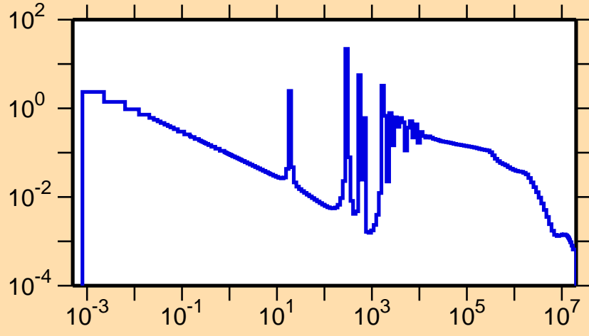
\sigma vs. E for ^{196}\text{Pt}(n,\gamma)
