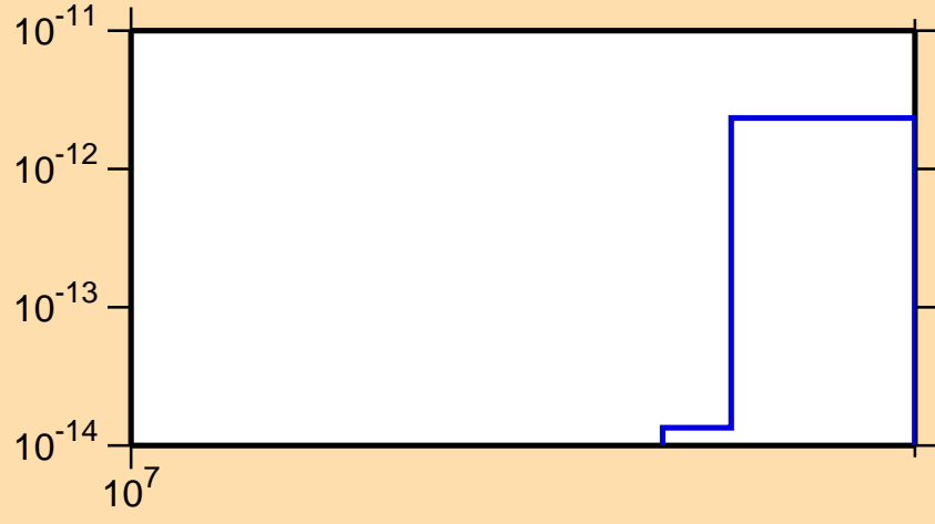
\sigma vs. E for ^{196}\text{Pt}(n,\text{He3})
