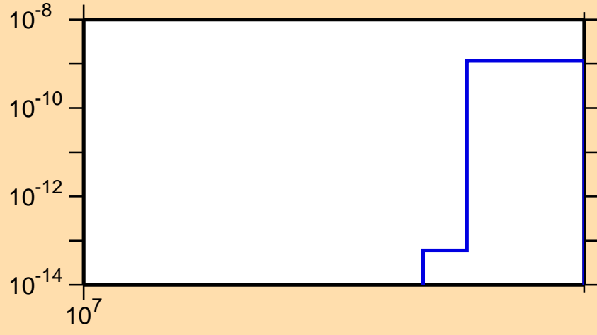
\sigma vs. E for ^{196}\text{Pt}(n,\text{nd})
