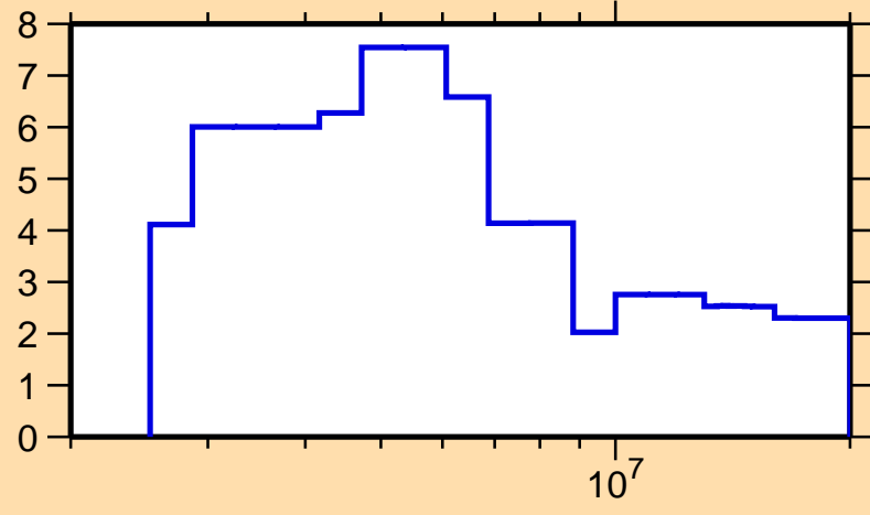
\Delta\sigma/\sigma vs. E for ^{196}\text{Pt}(n,\text{el.})
