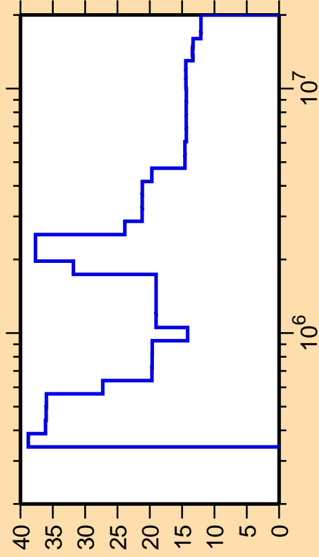
\Delta\sigma/\sigma vs. E for ^{196}\text{Pt}(n,n_1)
