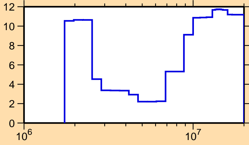
\Delta\sigma/\sigma vs. E for ^{196}\text{Pt}(n,\text{inel.})
