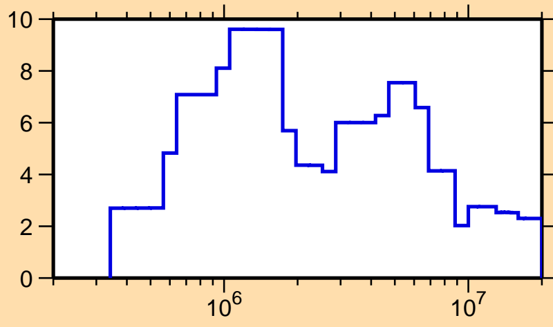
\Delta\sigma/\sigma vs. E for ^{196}\text{Pt}(n,\text{el.})
