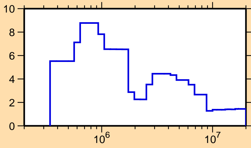
\Delta\sigma/\sigma vs. E for ^{196}\text{Pt}(n,\text{tot.})
