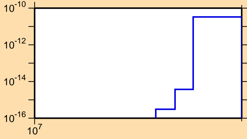
\sigma vs. E for ^{196}\text{Pt}(n,2np)
