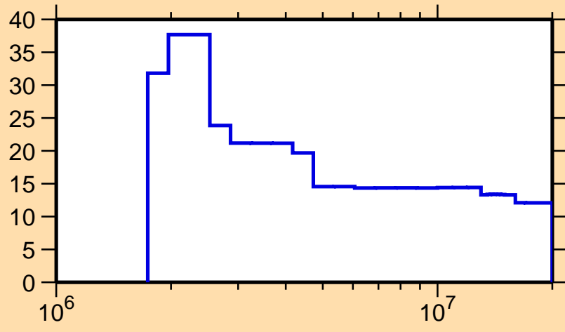
\Delta\sigma/\sigma vs. E for ^{196}\text{Pt}(n,n_1)
