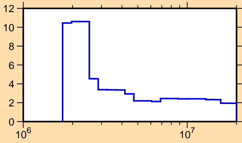
\Delta\sigma/\sigma vs. E for ^{196}\text{Pt}(n,\text{nonel.})
