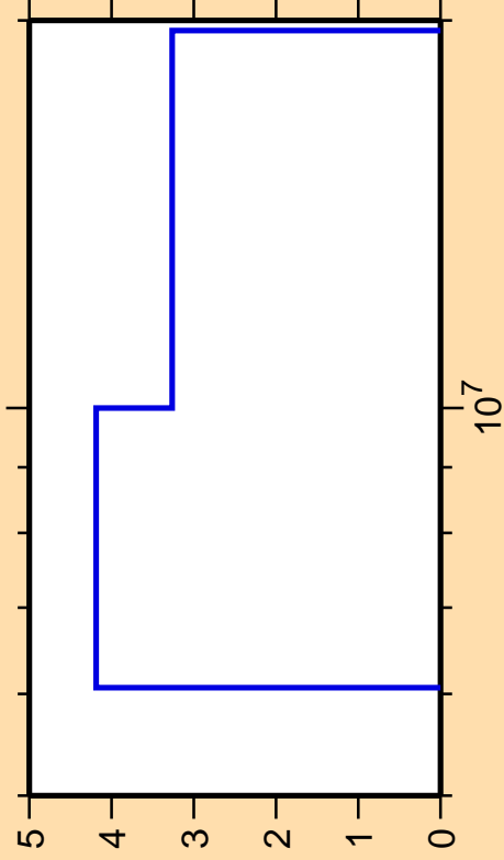
\Delta\sigma/\sigma vs. E for ^{196}\text{Pt}(n,2n)
