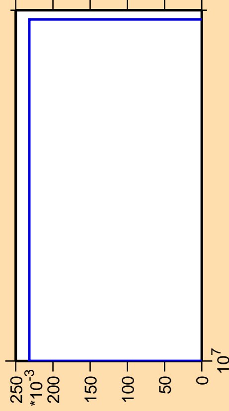
\Delta\sigma/\sigma vs. E for ^{196}\text{Pt}(n,2np)
