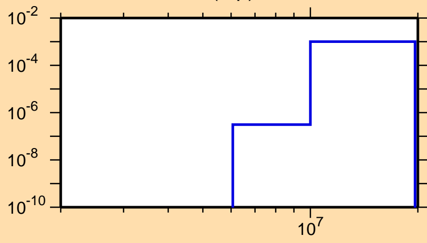
\sigma vs. E for ^{196}\text{Pt}(n,p)
