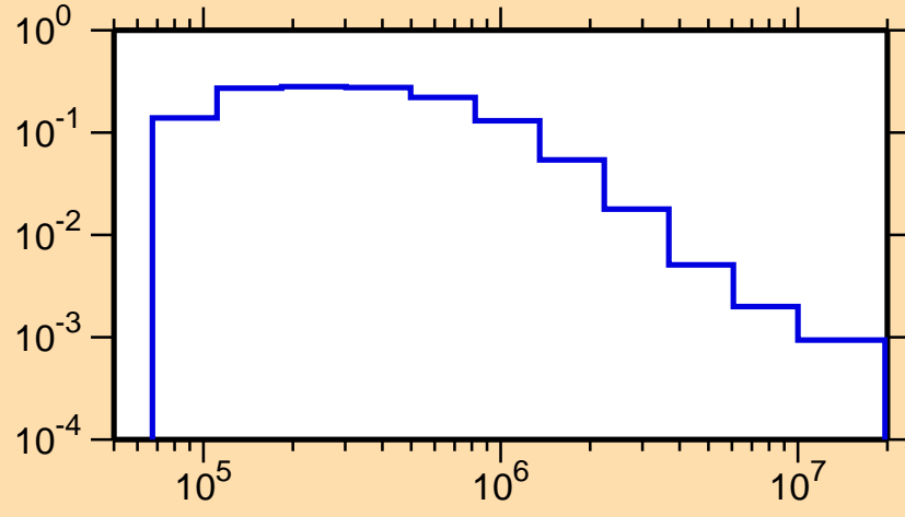
\sigma vs. E for ^{197}\text{Pt}(n,n_2)
