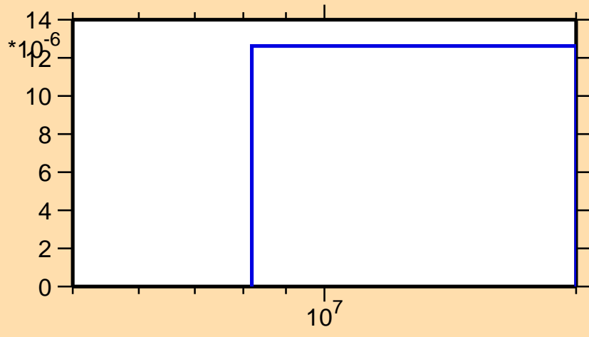
\sigma vs. E for ^{197}\text{Pt}(n,np)
