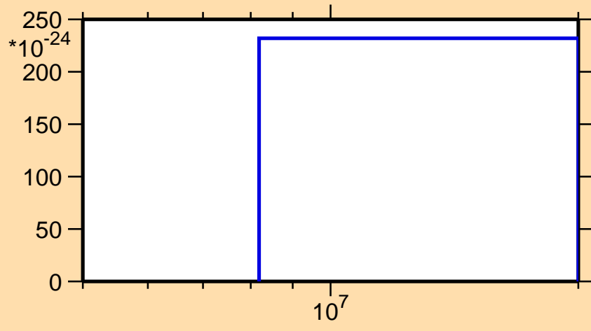
\sigma vs. E for ^{197}\text{Pt}(\text{mt } 11)
