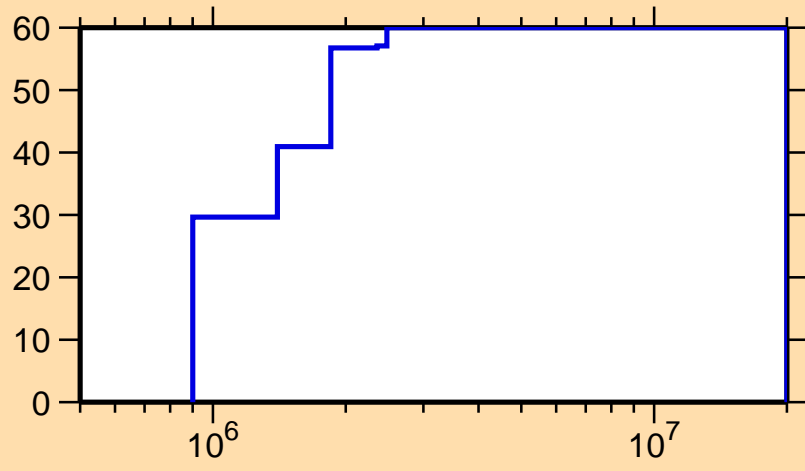
\Delta\sigma/\sigma vs. E for ^{197}\text{Pt}(n,n_1)
