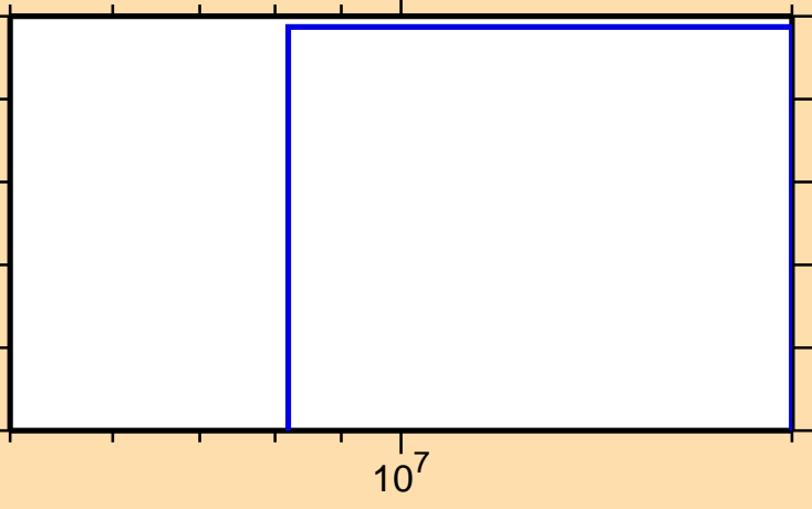
\sigma vs. E for ^{197}\text{Pt}(n,t)
