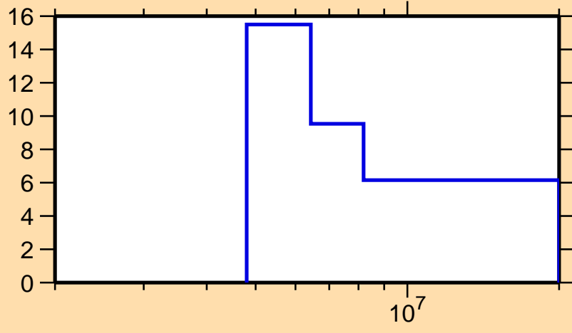
\Delta\sigma/\sigma vs. E for ^{197}\text{Pt}(n,2n)
