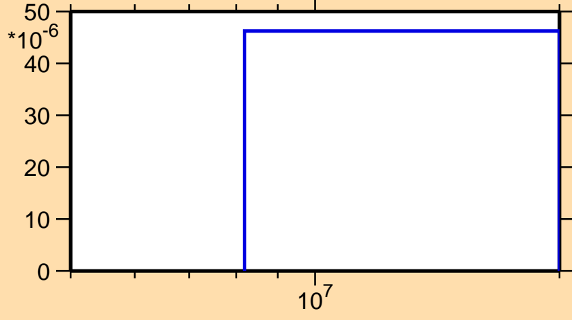
\sigma vs. E for ^{197}\text{Pt}(n,d)
