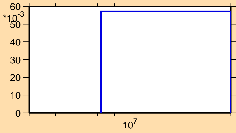
\sigma vs. E for ^{197}\text{Pt}(n,3n)
