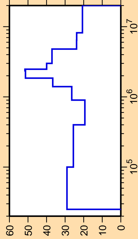
\Delta\sigma/\sigma vs. E for ^{197}\text{Pt}(n,n_2)
