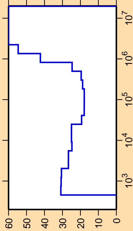
\Delta\sigma/\sigma vs. E for ^{197}\text{Pt}(n,n_3)
