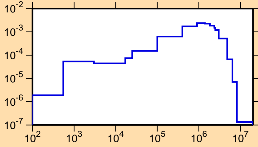
\sigma vs. E for ^{197}\text{Pt}(n,n_4)
