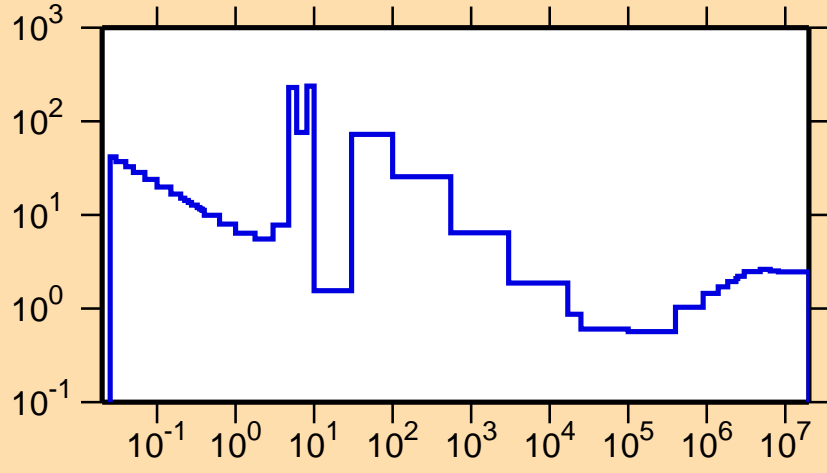
\sigma vs. E for ^{197}\text{Pt}(n,\text{nonel.})
