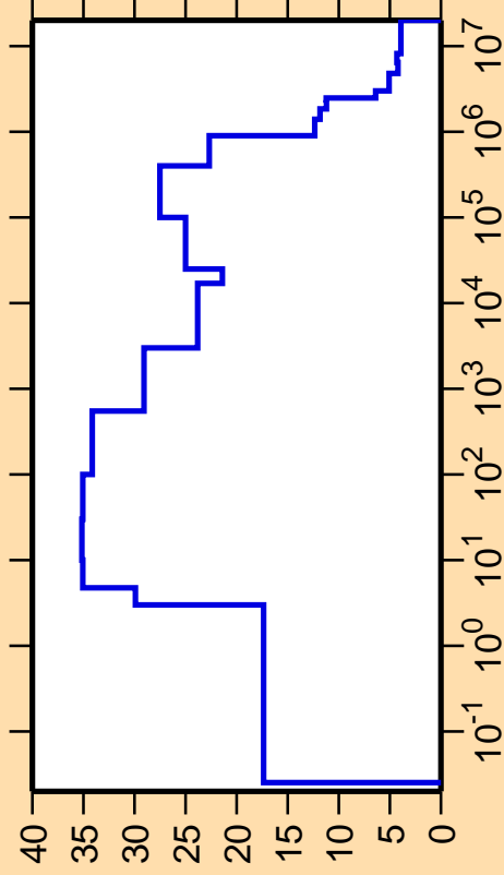
\Delta\sigma/\sigma vs. E for ^{197}\text{Pt}(n,\text{nonel.})
