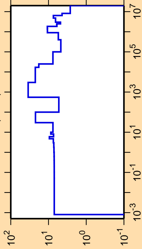
\Delta\sigma/\sigma vs. E for ^{197}\text{Pt}(n,\text{el.})
