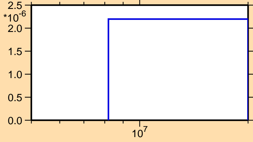
\sigma vs. E for ^{197}\text{Pt}(n,n\alpha)
