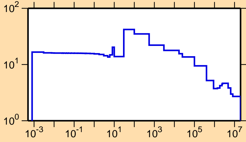
\sigma vs. E for ^{197}\text{Pt}(n,\text{el.})
