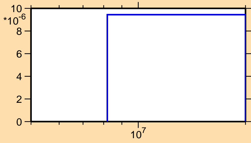
\sigma vs. E for ^{197}\text{Pt}(n,t)
