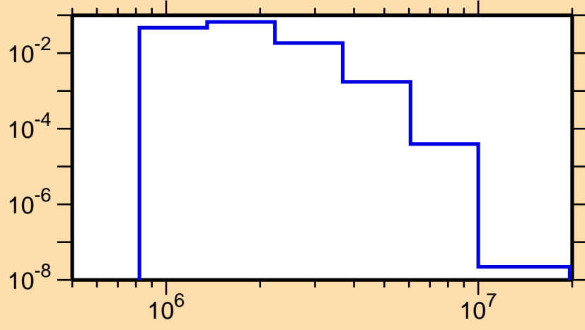
\sigma vs. E for ^{198}\text{Pt}(n,n_3)
