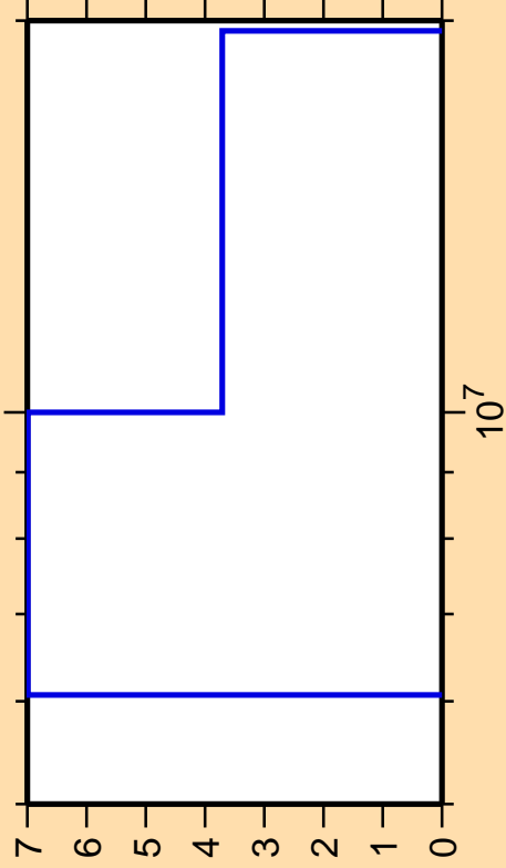
\Delta\sigma/\sigma vs. E for ^{198}\text{Pt}(n,2n)
