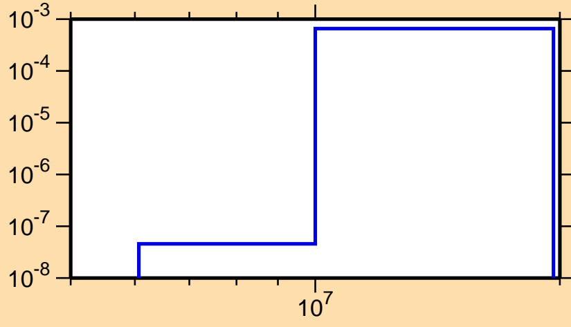
\sigma vs. E for ^{198}\text{Pt}(n,p)
