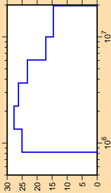
\Delta\sigma/\sigma vs. E for ^{198}\text{Pt}(n,n_4)
