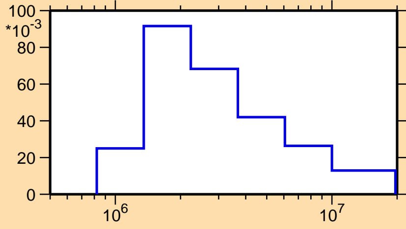
\sigma vs. E for ^{198}\text{Pt}(n,n_4)
