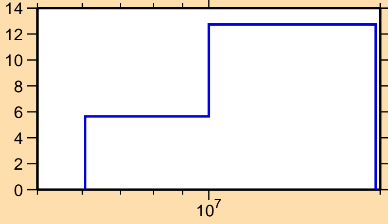
\Delta\sigma/\sigma vs. E for ^{198}\text{Pt}(n,ncont.)
