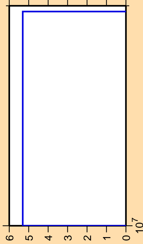
\Delta\sigma/\sigma vs. E for ^{199}\text{Pt}(n,2np)
