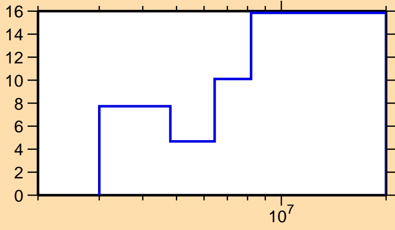
\Delta\sigma/\sigma vs. E for ^{199}\text{Pt}(n,ncont.)
