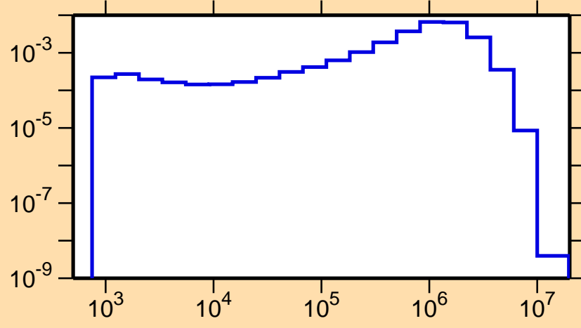
\sigma vs. E for ^{199}\text{Pt}(n,n_3)
