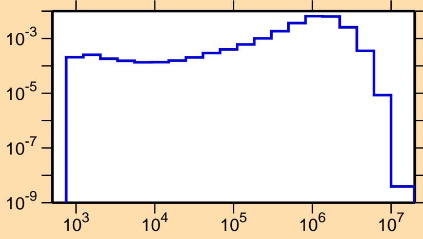
\sigma vs. E for ^{199}\text{Pt}(n,n_4)
