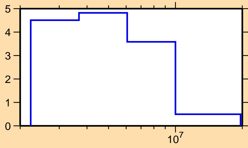
\Delta\sigma/\sigma vs. E for ^{199}\text{Pt}(n,\text{tot.})
