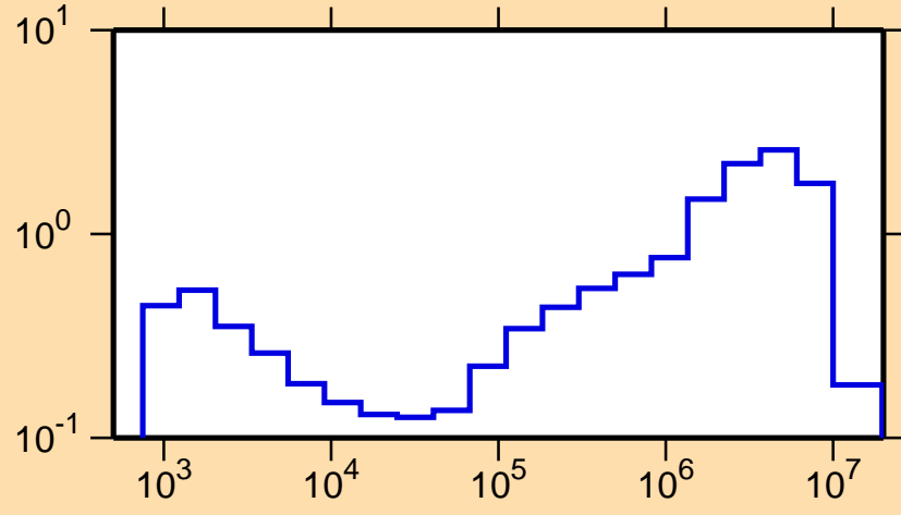
\sigma vs. E for ^{199}\text{Pt}(n,\text{inel.})
