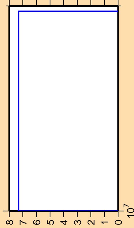
\Delta\sigma/\sigma vs. E for ^{199}\text{Pt}(n,3n)
