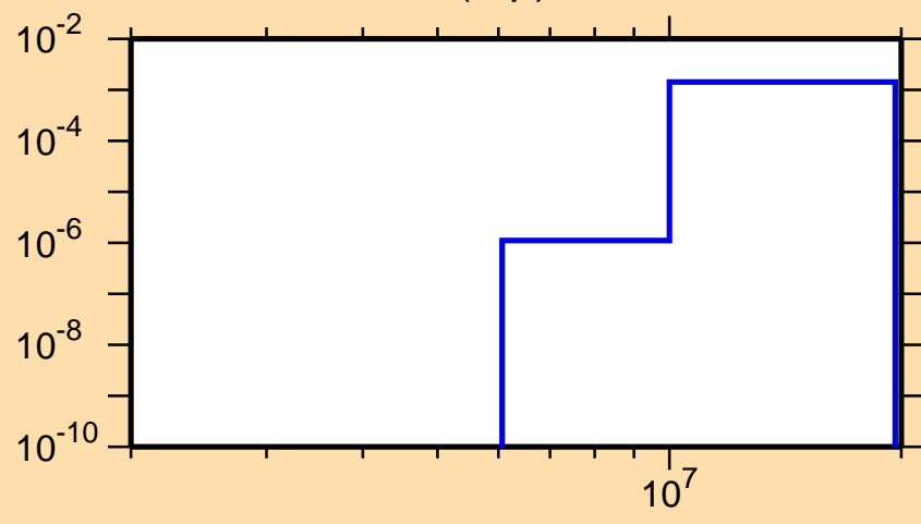
\sigma vs. E for ^{199}\text{Pt}(n,p)
