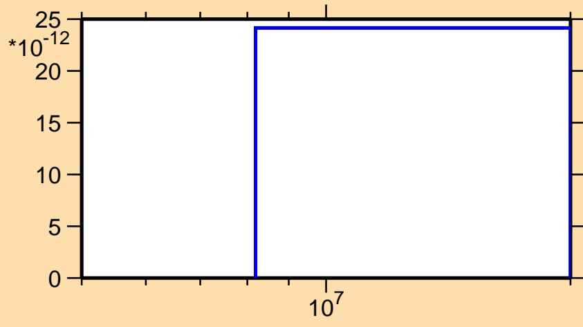
\sigma vs. E for ^{199}\text{Pt}(n,nt)
