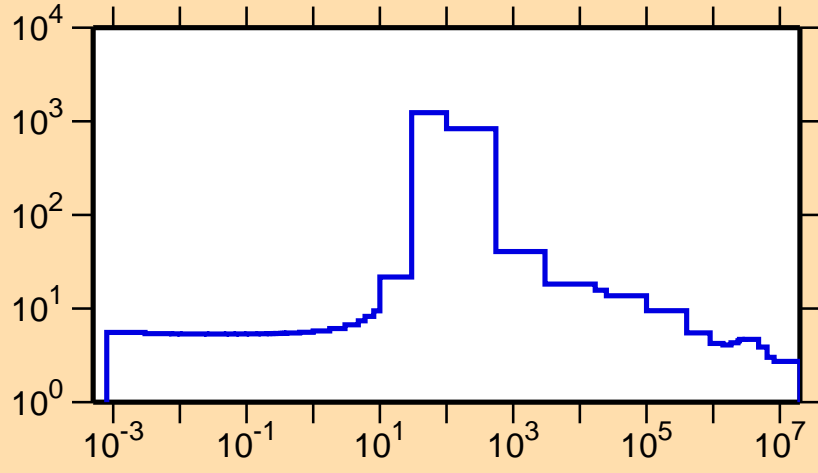
\sigma vs. E for ^{199}\text{Pt}(n,\text{el.})
