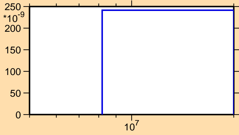
\sigma vs. E for ^{199}\text{Pt}(n,n\alpha)
