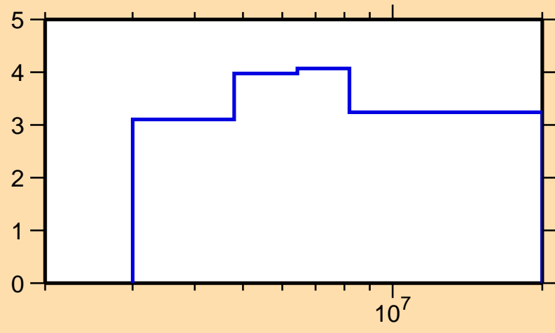
\Delta\sigma/\sigma vs. E for ^{199}\text{Pt}(n,\text{nonel.})
