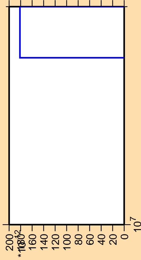
\Delta\sigma/\sigma vs. E for ^{200}\text{Pt}(\text{mt } 11)
