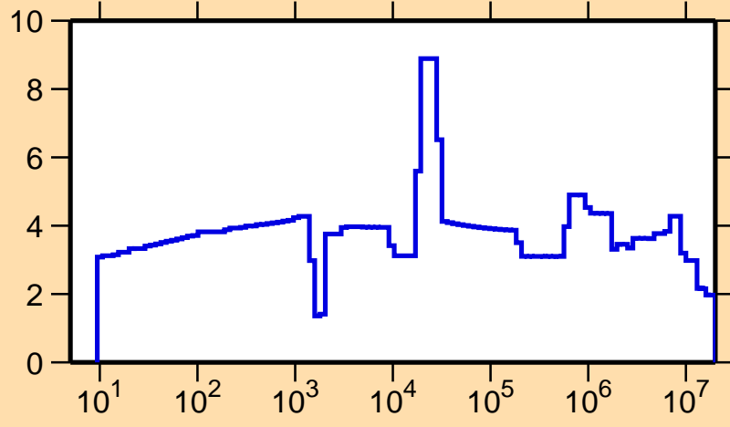
\Delta\sigma/\sigma vs. E for ^{200}\text{Pt}(n,\text{tot.})
