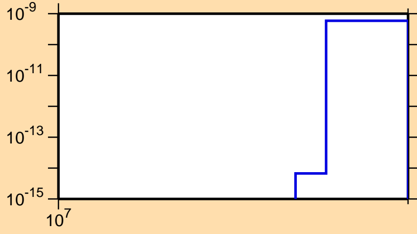
\sigma vs. E for ^{200}\text{Pt}(n,nt)
