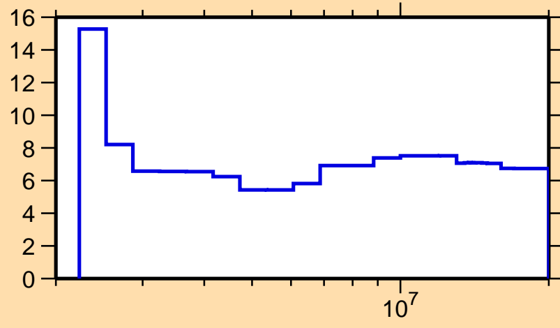
\Delta\sigma/\sigma vs. E for ^{200}\text{Pt}(n,\text{nonel.})
