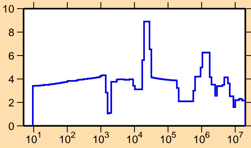
\Delta\sigma/\sigma vs. E for ^{200}\text{Pt}(n,\text{el.})
