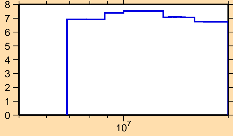
\Delta\sigma/\sigma vs. E for ^{200}\text{Pt}(n,\text{nonel.})
