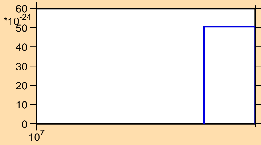
\sigma vs. E for ^{200}\text{Pt}(\text{mt } 11)
