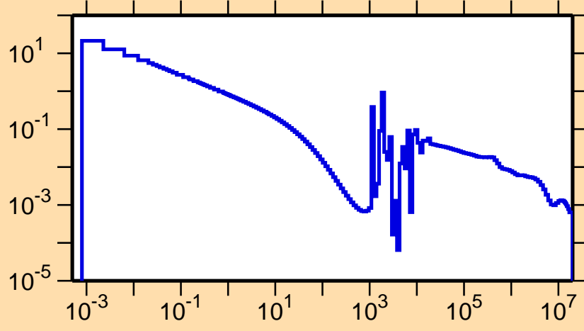
\sigma vs. E for ^{200}\text{Pt}(n,\gamma)
