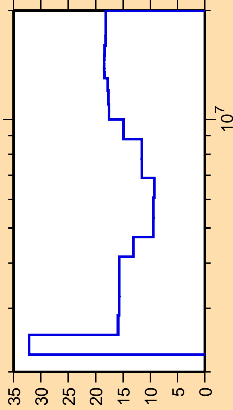
\Delta\sigma/\sigma vs. E for ^{200}\text{Pt}(n,n\text{cont.})
