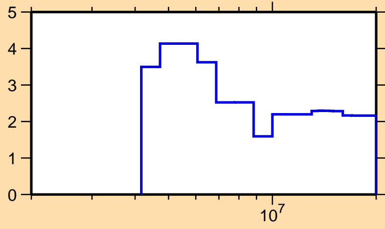
\Delta\sigma/\sigma vs. E for ^{200}\text{Pt}(n,\text{el.})
