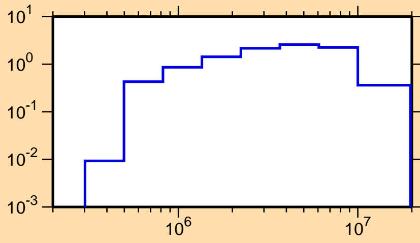
\sigma vs. E for ^{200}\text{Pt}(n,\text{inel.})
