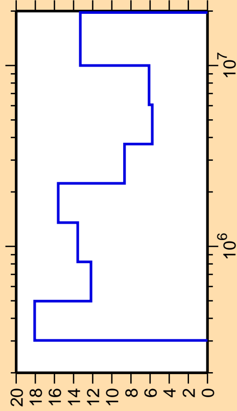
\Delta\sigma/\sigma vs. E for ^{200}\text{Pt}(n,\text{inel.})
