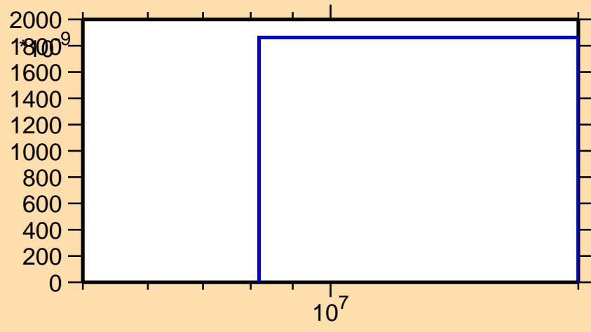
\sigma vs. E for ^{200}\text{Pt}(n,np)
