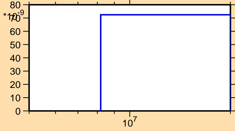
\sigma vs. E for ^{200}\text{Pt}(n,n\alpha)
