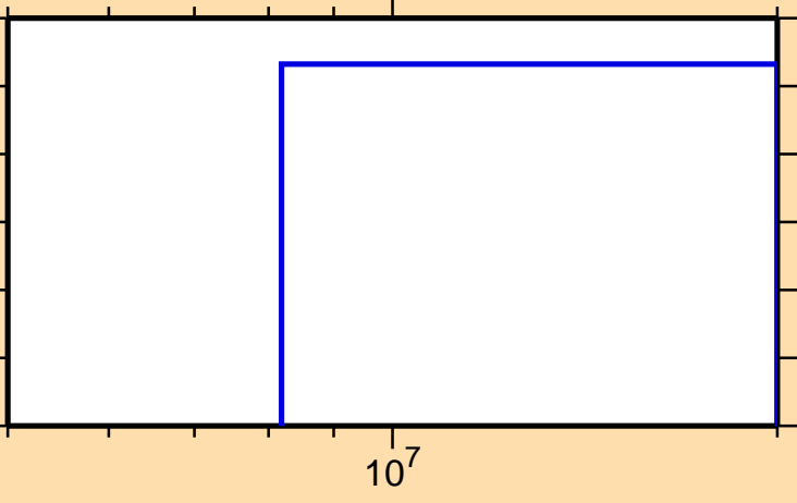
\sigma vs. E for ^{200}\text{Pt}(n,t)
