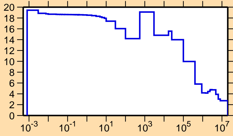
\sigma vs. E for ^{200}\text{Pt}(n,\text{el.})
