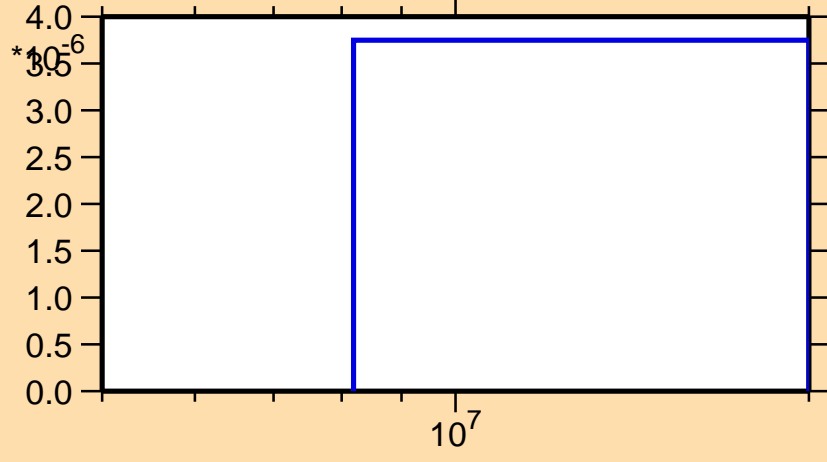
\sigma vs. E for ^{200}\text{Pt}(n,d)
