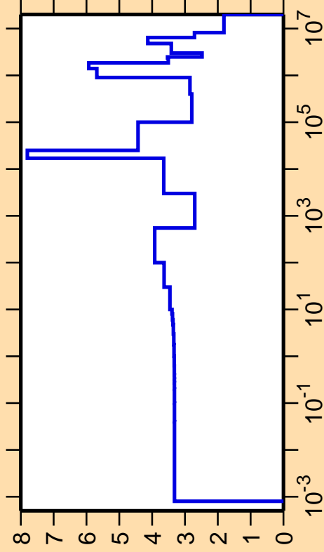
\Delta\sigma/\sigma vs. E for ^{200}\text{Pt}(n,\text{el.})
