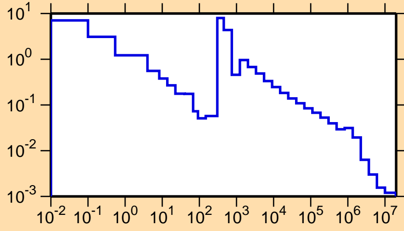
\sigma vs. E for ^{201}\text{Pt}(n,\gamma)
