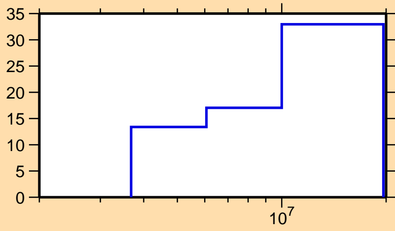
\Delta\sigma/\sigma vs. E for ^{201}\text{Pt}(n,n\text{cont.})
