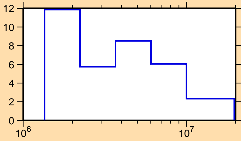
\Delta\sigma/\sigma vs. E for ^{201}\text{Pt}(n,\text{tot.})
