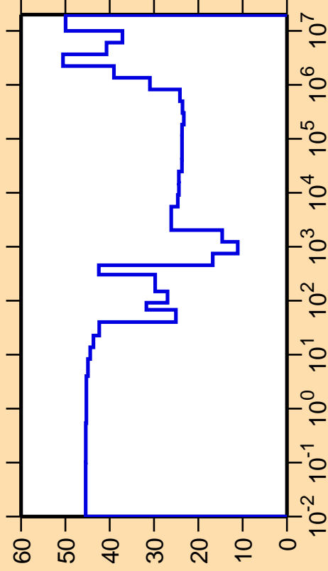
\Delta\sigma/\sigma vs. E for ^{201}\text{Pt}(n,\gamma)
