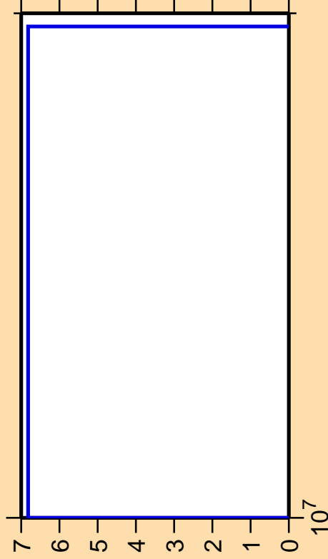
\Delta\sigma/\sigma vs. E for ^{201}\text{Pt}(n,2n\alpha)
