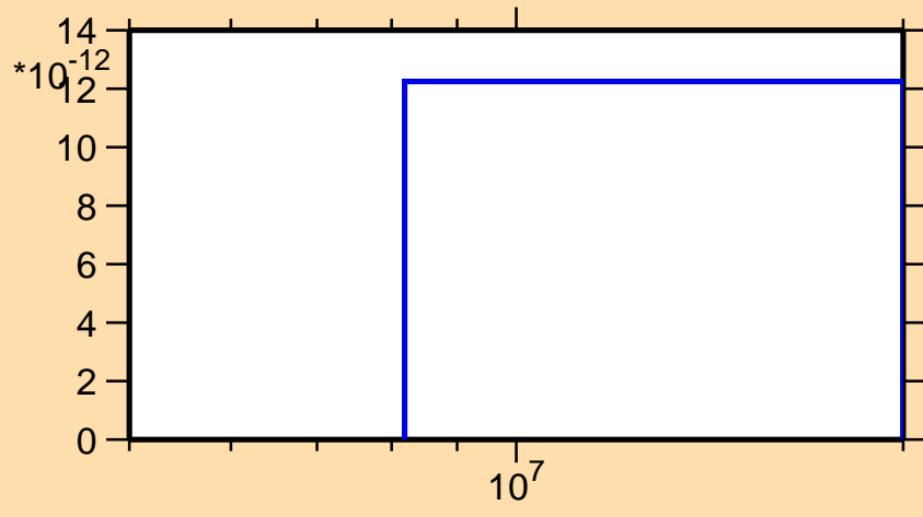
\sigma vs. E for ^{201}\text{Pt}(n,nt)
