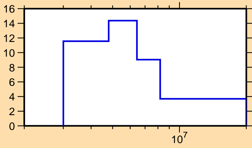
\Delta\sigma/\sigma vs. E for ^{201}\text{Pt}(n,el.)
