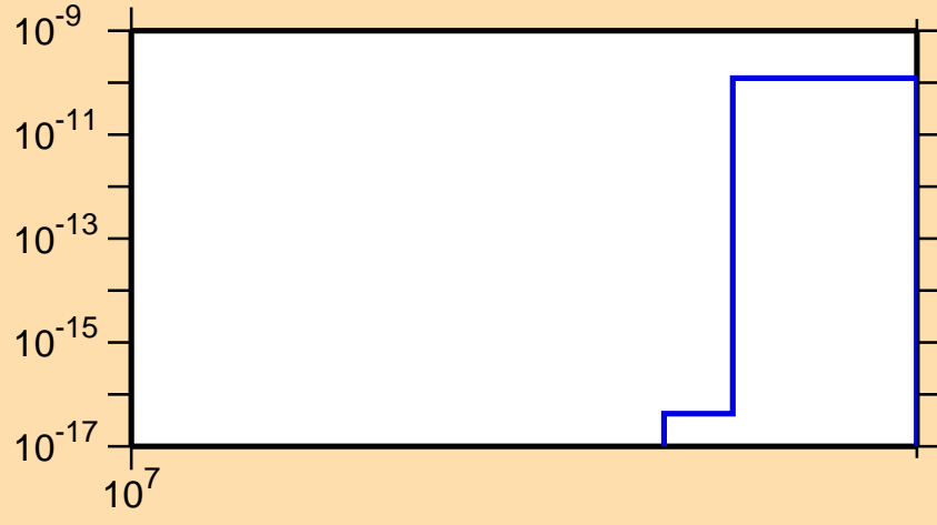
\sigma vs. E for ^{202}\text{Pt}(n,\text{nd})
