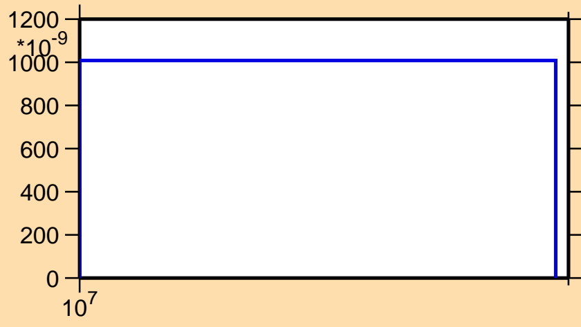
\sigma vs. E for ^{202}\text{Pt}(n,np)
