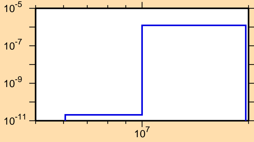
\sigma vs. E for ^{202}\text{Pt}(n,\alpha)
