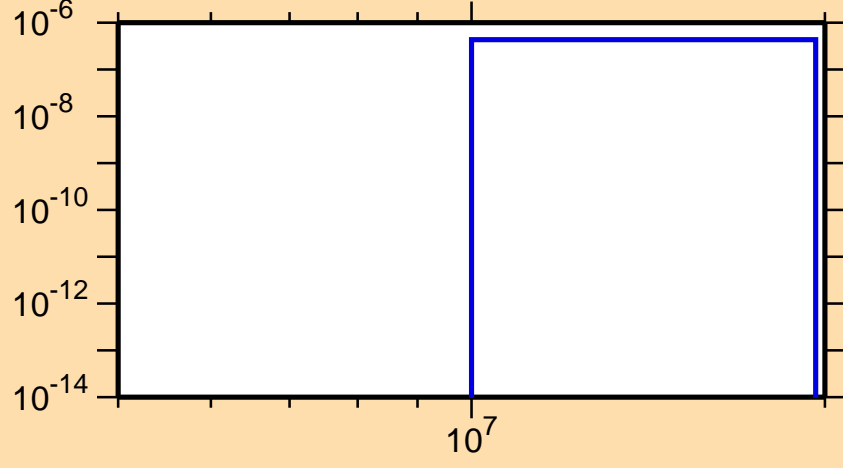
\sigma vs. E for ^{202}\text{Pt}(n,t)
