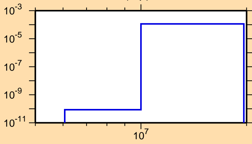
\sigma vs. E for ^{202}\text{Pt}(n,p)
