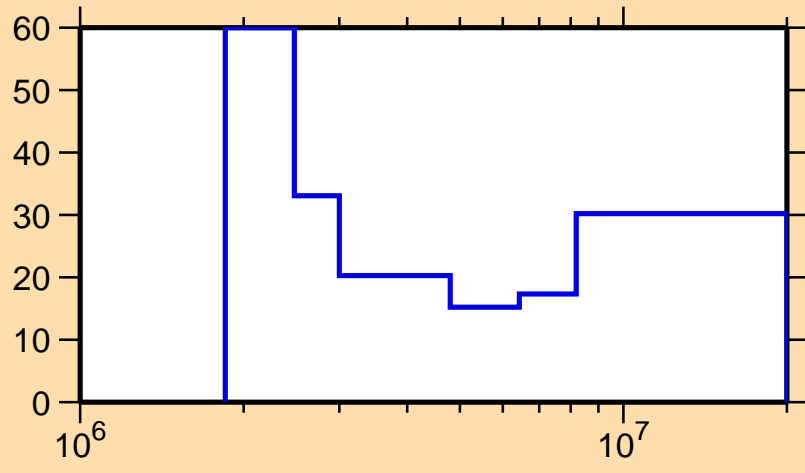
\Delta\sigma/\sigma vs. E for ^{202}\text{Pt}(n,n\text{cont.})
