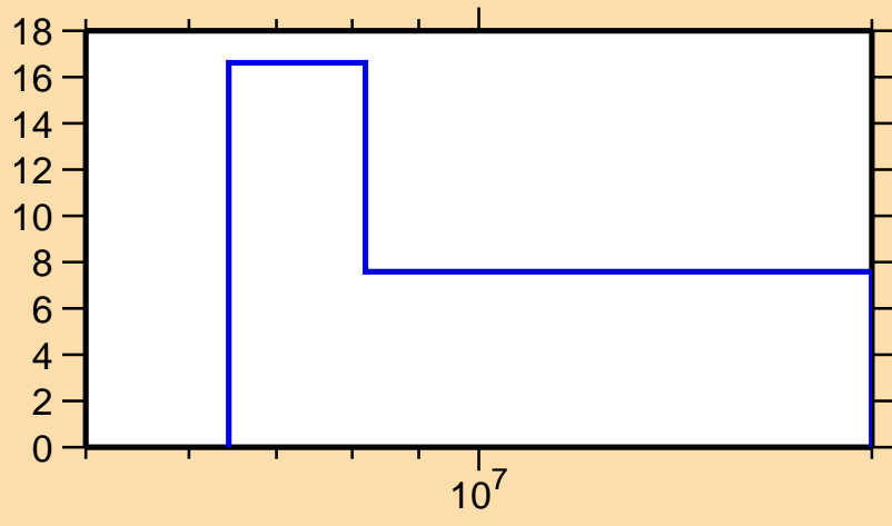
\Delta\sigma/\sigma vs. E for ^{202}\text{Pt}(n,el.)
