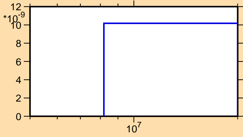
\sigma vs. E for ^{202}\text{Pt}(n,n\alpha)
