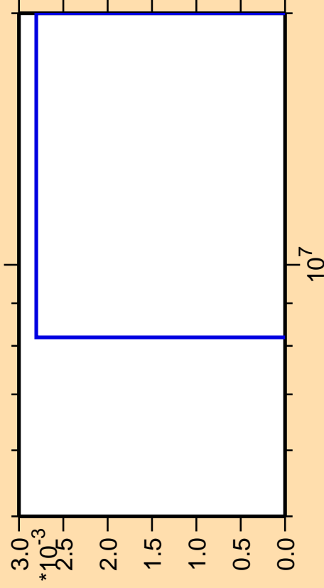
\Delta\sigma/\sigma vs. E for ^{202}\text{Pt}(n,2np)
