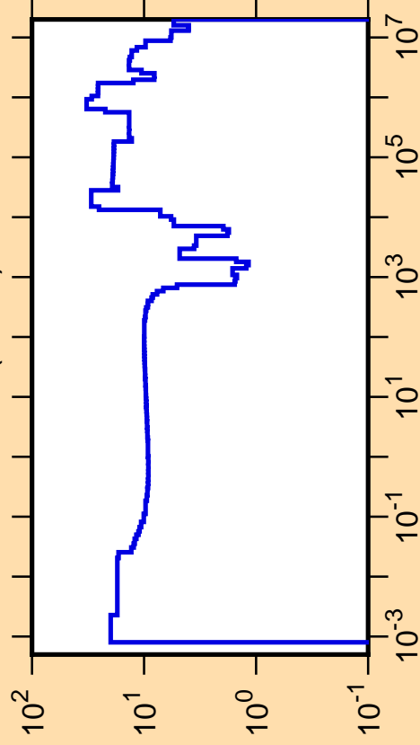
\Delta\sigma/\sigma vs. E for ^{203}\text{Pt}(n,\text{tot.})
