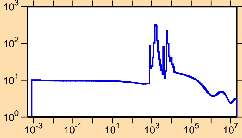
\sigma vs. E for ^{203}\text{Pt}(n,\text{el.})
