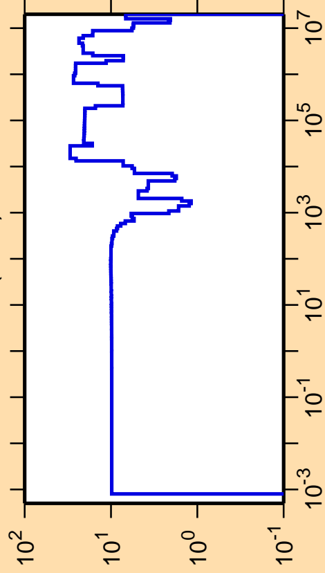
\Delta\sigma/\sigma vs. E for ^{203}\text{Pt}(n,\text{el.})
