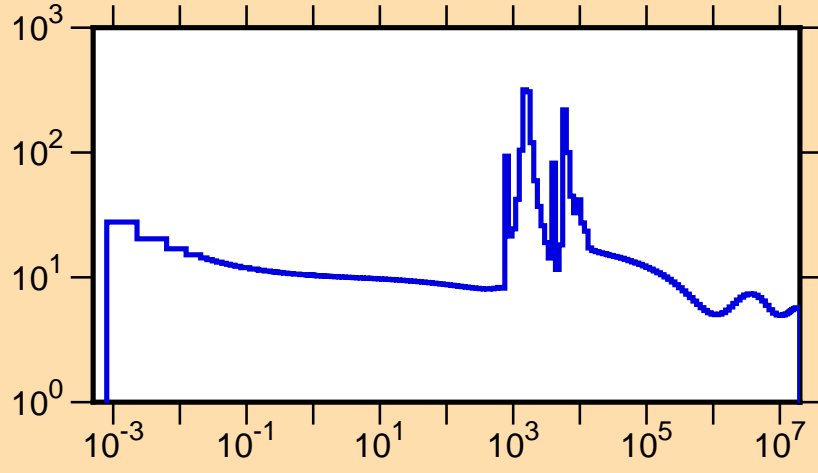
\sigma vs. E for ^{203}\text{Pt}(n,\text{tot.})
