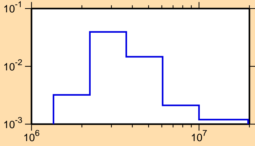
\sigma vs. E for ^{204}\text{Pt}(n,n_4)
