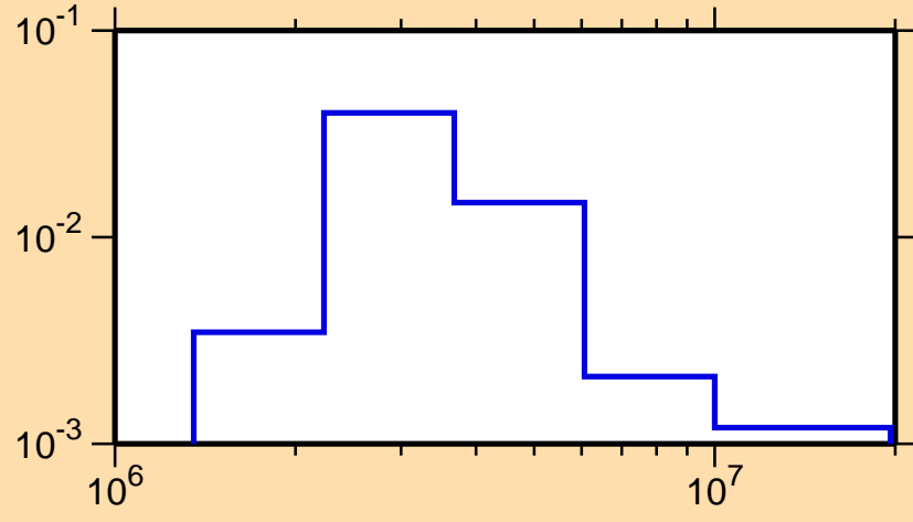
\sigma vs. E for ^{204}\text{Pt}(n,n_2)
