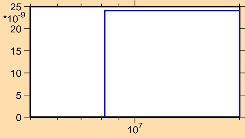
\sigma vs. E for ^{204}\text{Pt}(n,n\alpha)
