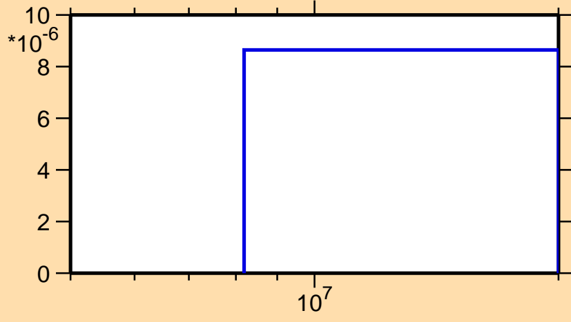
\sigma vs. E for ^{204}\text{Pt}(n,p)
