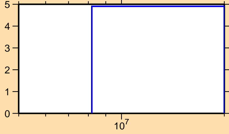
\Delta\sigma/\sigma vs. E for ^{204}\text{Pt}(n,el.)
