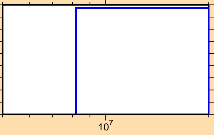
\sigma vs. E for ^{205}\text{Pt}(\text{mt } 42)
