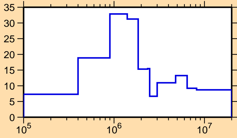
\Delta\sigma/\sigma vs. E for ^{205}\text{Pt}(n, el.)
