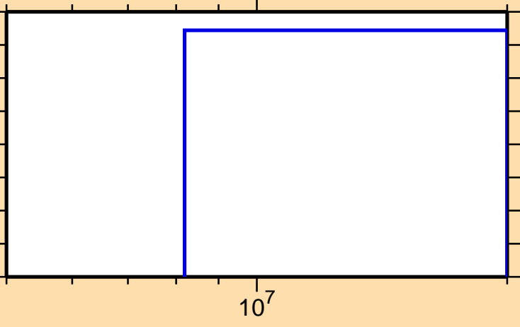
\sigma vs. E for ^{205}\text{Pt}(n,t)
