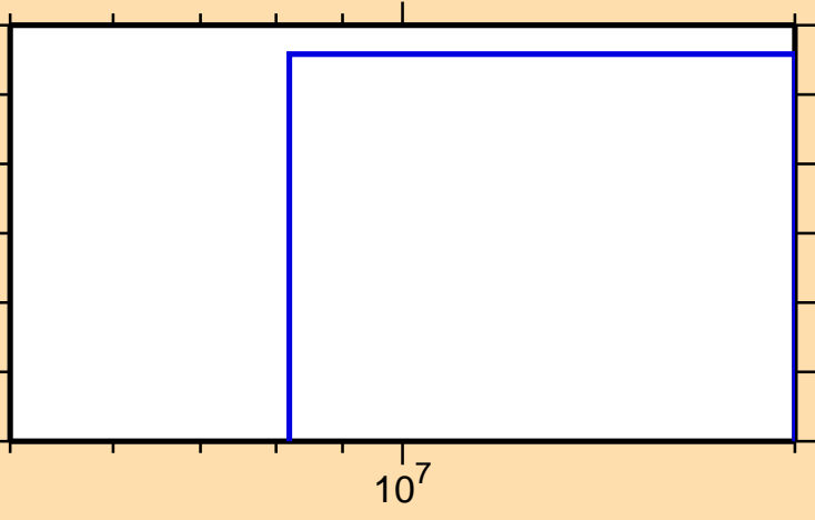
\sigma vs. E for ^{205}\text{Pt}(n,2np)
