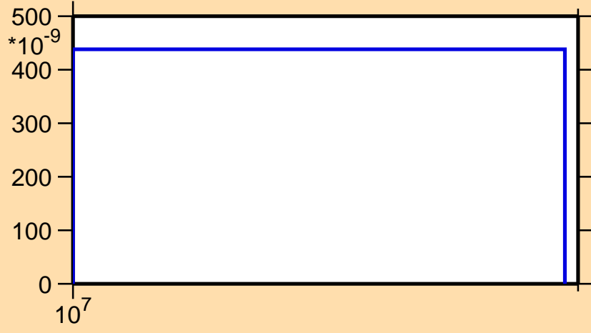
\sigma vs. E for ^{206}\text{Pt}(n,d)
