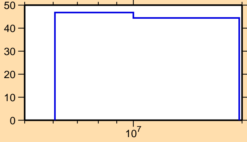
\Delta\sigma/\sigma vs. E for ^{206}\text{Pt}(n,n_1)
