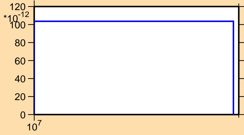
\sigma vs. E for ^{206}\text{Pt}(n,\text{nd})
