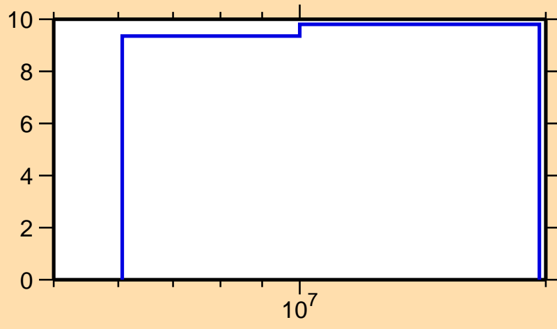
\Delta\sigma/\sigma vs. E for ^{206}\text{Pt}(n,\text{nonel.})
