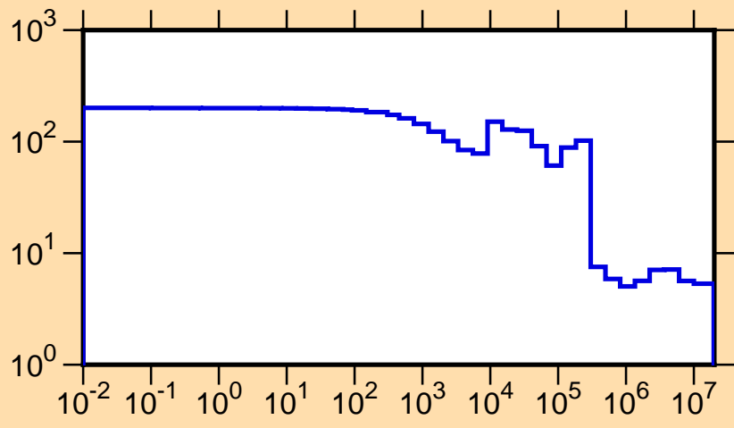
\sigma vs. E for ^{206}\text{Pt}(n,\text{tot.})
