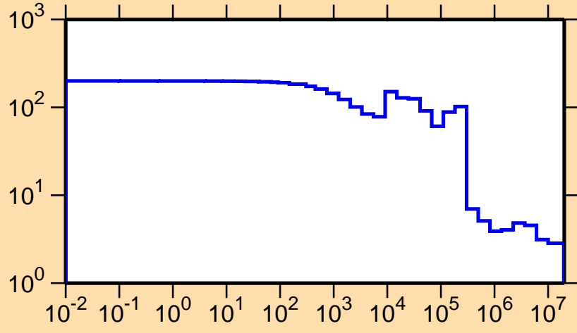
\sigma vs. E for ^{206}\text{Pt}(n,\text{el.})
