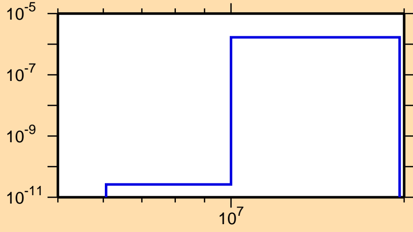
\sigma vs. E for ^{206}\text{Pt}(n,\alpha)
