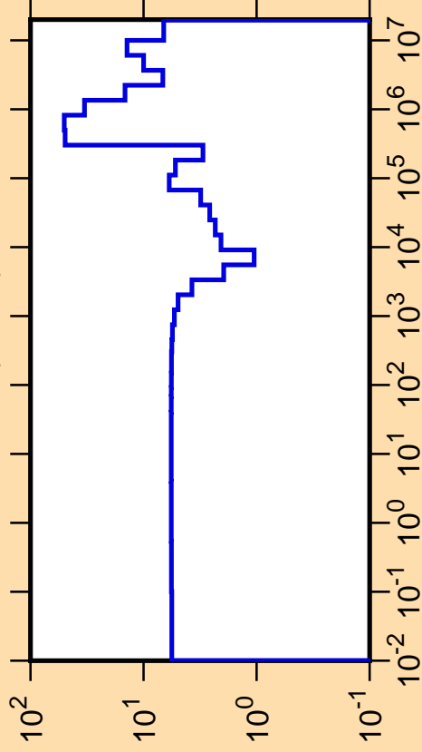
\Delta\sigma/\sigma vs. E for ^{206}\text{Pt}(n,\text{tot.})
