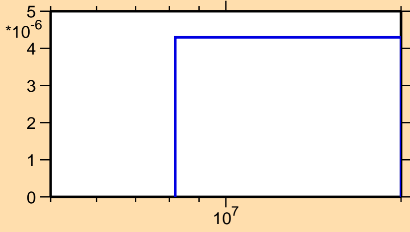
\sigma vs. E for ^{206}\text{Pt}(n,t)
