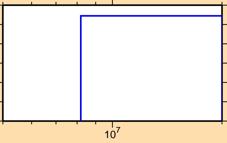
\sigma vs. E for ^{206}\text{Pt}(n,nt)
