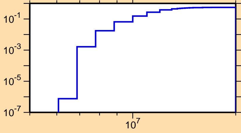
\sigma vs. E for ^{229}\text{Pu}(n,2n)
