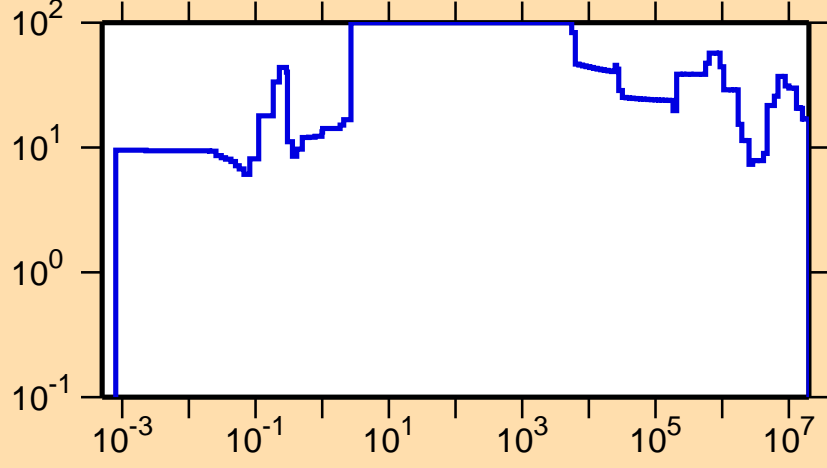
\Delta\sigma/\sigma vs. E for ^{229}\text{Pu}(n,tot.)
