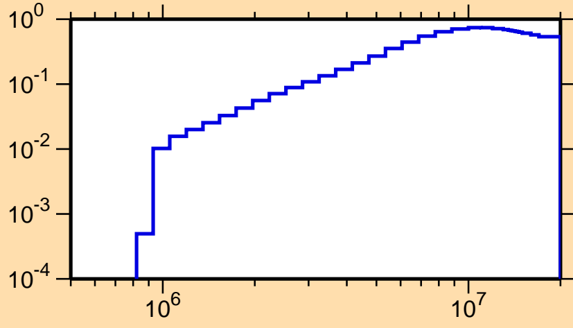
\sigma vs. E for ^{229}\text{Pu}(n,n\text{cont.})
