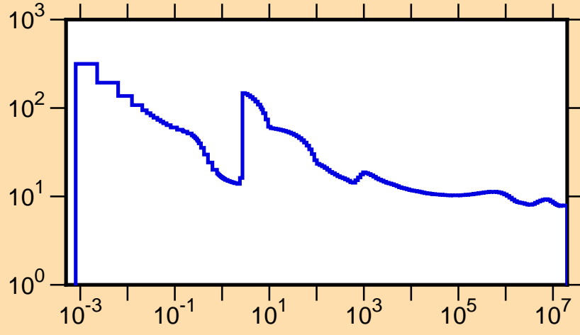
\sigma vs. E for ^{229}\text{Pu}(n,\text{tot.})
