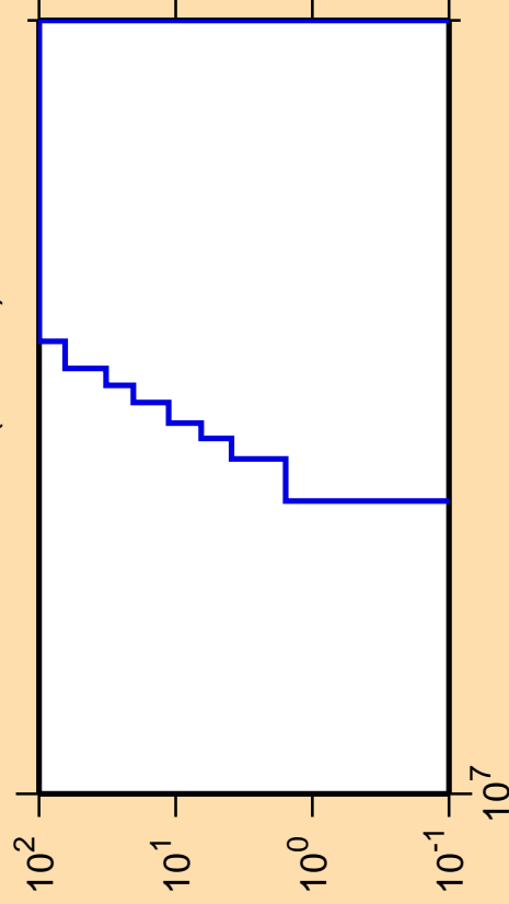
\Delta\sigma/\sigma vs. E for ^{229}\text{Pu}(\text{mt } 45)
