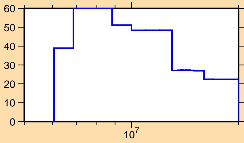
\Delta\sigma/\sigma vs. E for ^{229}\text{Pu}(n,\text{el.})
