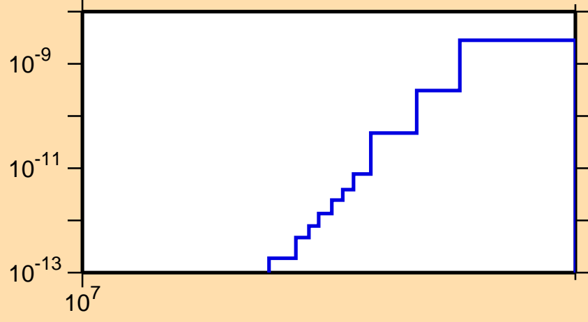
\sigma vs. E for ^{229}\text{Pu}(\text{mt } 45)
