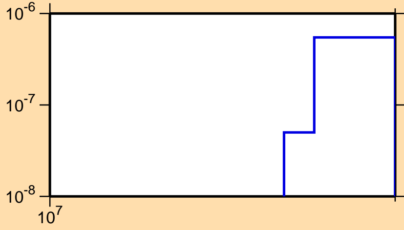
\sigma vs. E for ^{229}\text{Pu}(n,3n\alpha)
