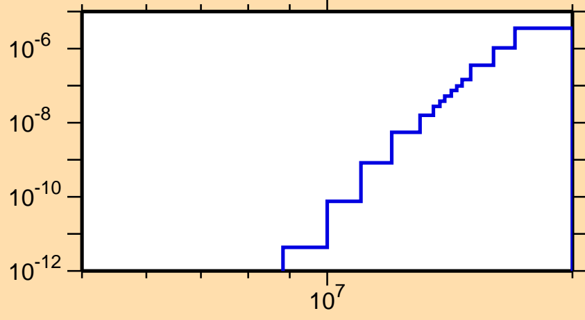
\sigma vs. E for ^{229}\text{Pu}(n,\text{He}3)
