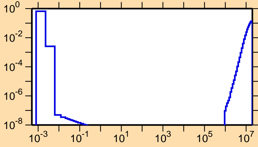
\sigma vs. E for ^{229}\text{Pu}(n,p)
