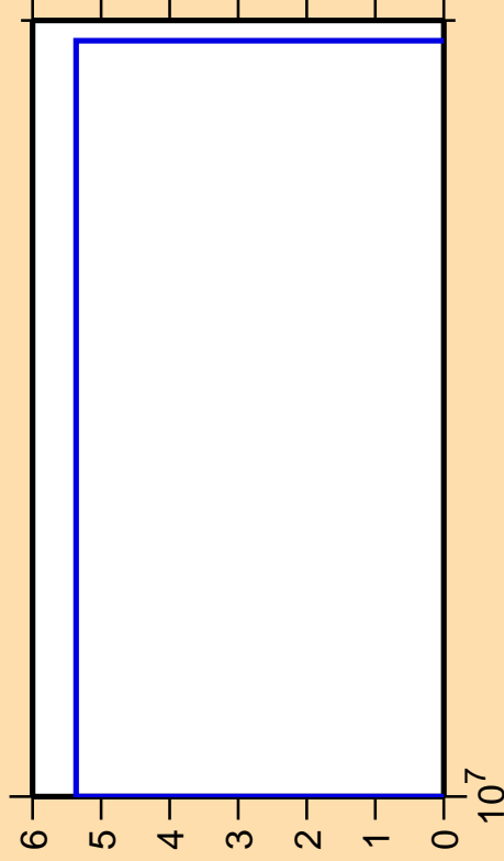
\Delta\sigma/\sigma vs. E for ^{229}\text{Pu}(n,\text{pd})
