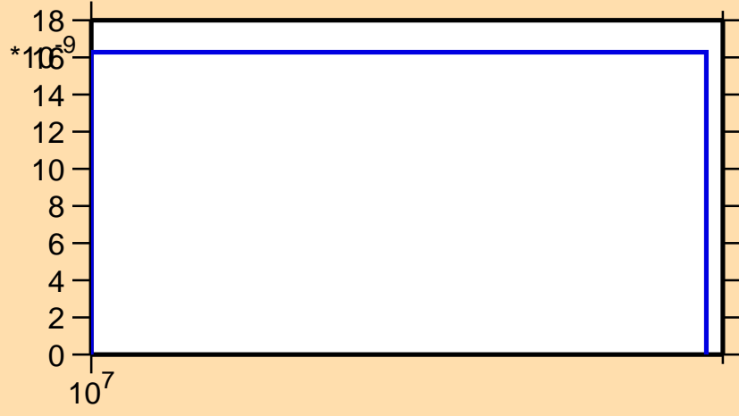
\sigma vs. E for ^{229}\text{Pu}(n,2np)
