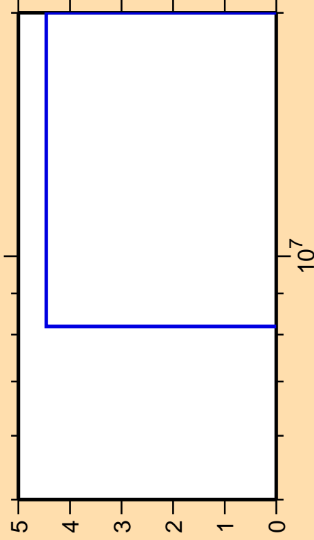
\Delta\sigma/\sigma vs. E for ^{229}\text{Pu}(n,pd)
