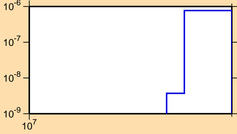
\sigma vs. E for ^{230}\text{Pu}(n,2np)
