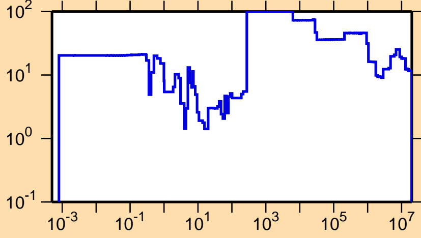
\Delta\sigma/\sigma vs. E for ^{230}\text{Pu}(n,\text{tot.})
