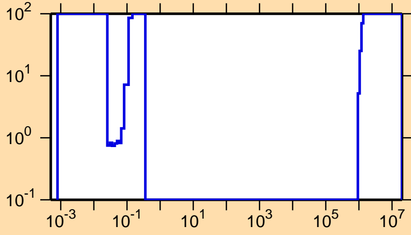
\Delta\sigma/\sigma vs. E for ^{230}\text{Pu}(n,p)
