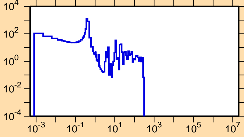
\sigma vs. E for ^{230}\text{Pu}(n,\gamma)
