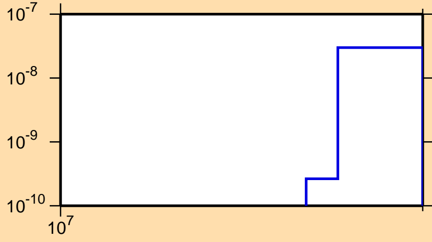
\sigma vs. E for ^{230}\text{Pu}(n,nt)
