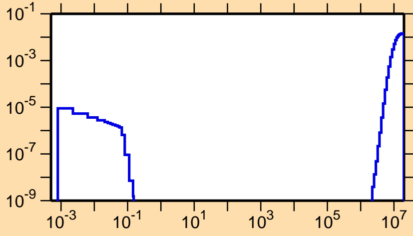
\sigma vs. E for ^{230}\text{Pu}(n,p)
