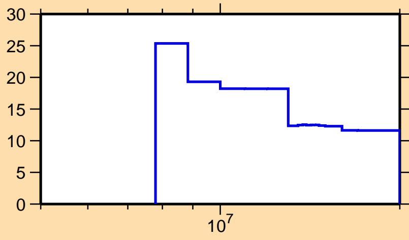
\Delta\sigma/\sigma vs. E for ^{230}\text{Pu}(n,\text{tot.})
