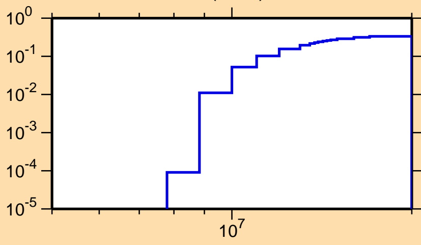
\sigma vs. E for ^{230}\text{Pu}(n,2n)
