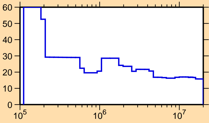
\Delta\sigma/\sigma vs. E for ^{230}\text{Pu}(n,\text{nonel.})
