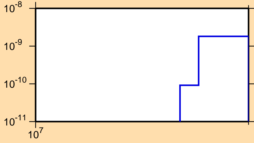
\sigma vs. E for ^{230}\text{Pu} (mt 45)
