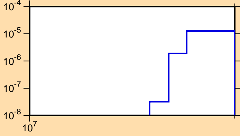
\sigma vs. E for ^{230}\text{Pu}(n,3n)
