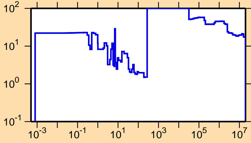
\Delta\sigma/\sigma vs. E for ^{230}\text{Pu}(n,f)
