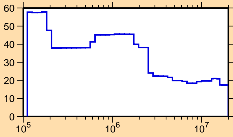
\Delta\sigma/\sigma vs. E for ^{230}\text{Pu}(n,f)
