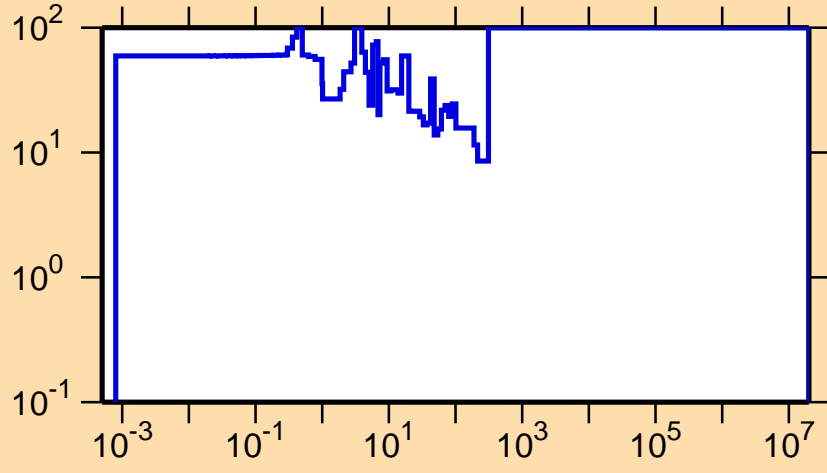
\Delta\sigma/\sigma vs. E for ^{230}\text{Pu}(n,\gamma)
