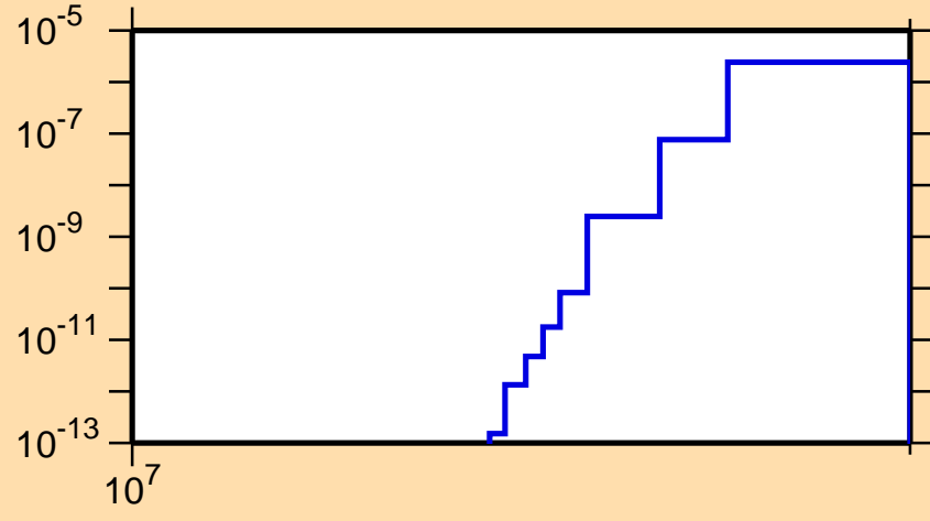
\sigma vs. E for ^{230}\text{Pu}(n,\text{nd})
