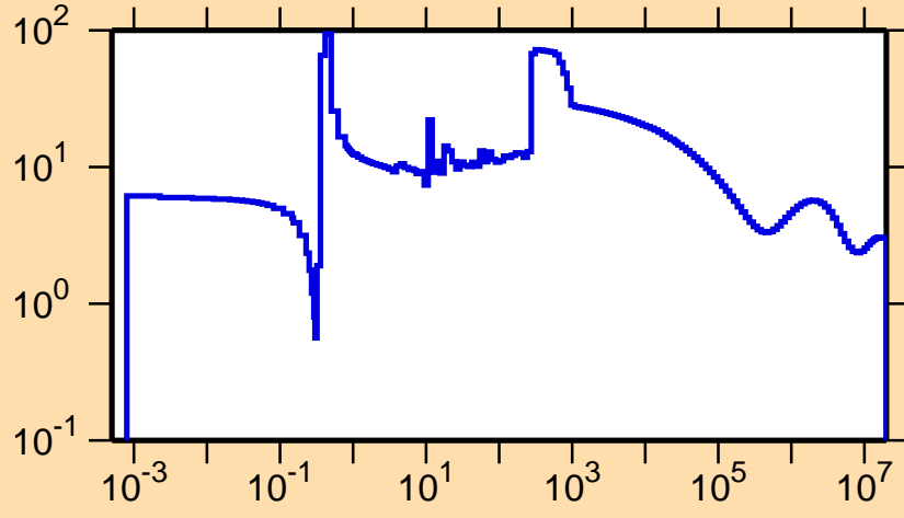
\sigma vs. E for ^{230}\text{Pu}(n,\text{el.})
