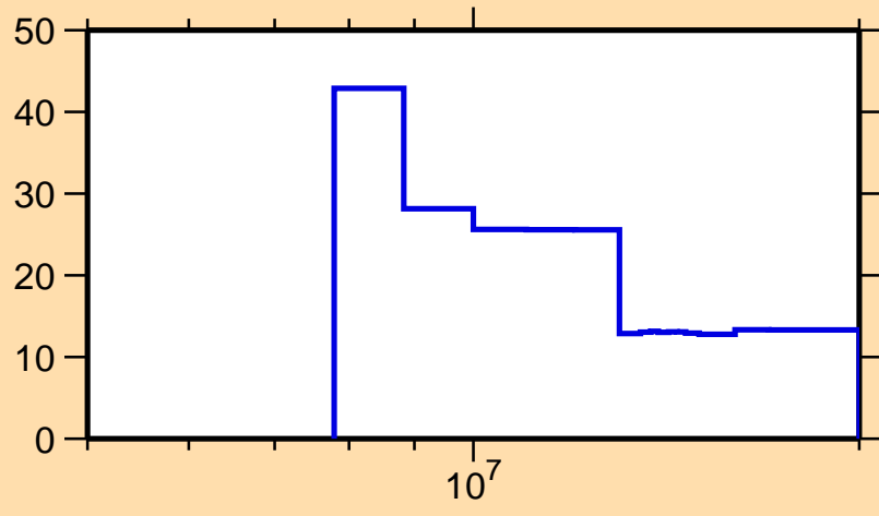
\Delta\sigma/\sigma vs. E for ^{230}\text{Pu}(n,\text{el.})
