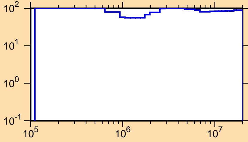
\Delta\sigma/\sigma vs. E for ^{230}\text{Pu}(n,n_1)
