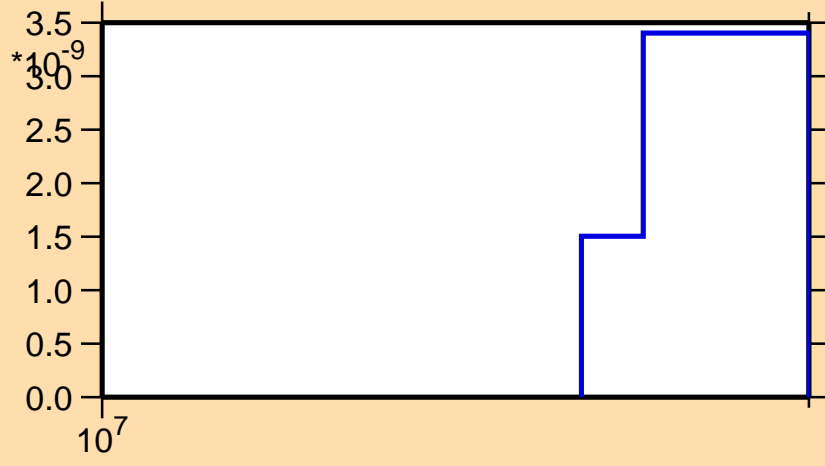
\sigma vs. E for ^{230}\text{Pu}(n,3n\alpha)
