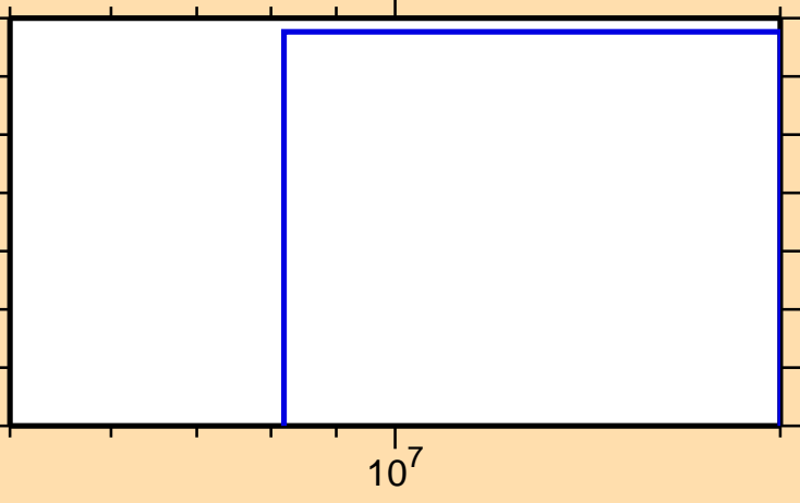
\sigma vs. E for ^{230}\text{Pu}(\text{mt117})
