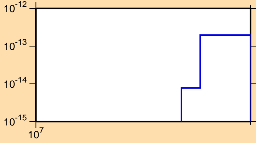
\sigma vs. E for ^{231}\text{Pu}(n,\text{pd})
