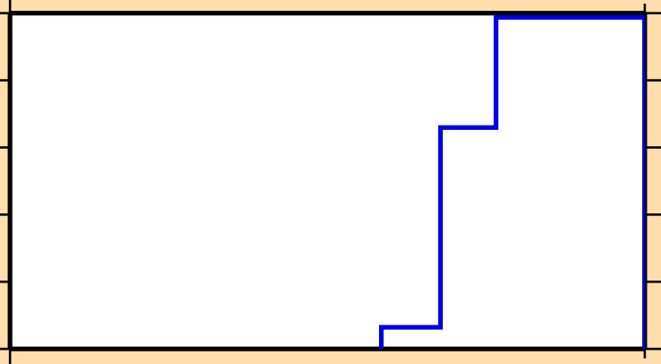
\sigma vs. E for ^{231}\text{Pu}(n,3n)
