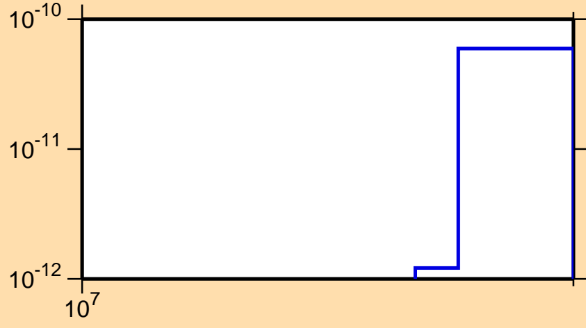
\sigma vs. E for ^{231}\text{Pu}(\text{mt 34})
