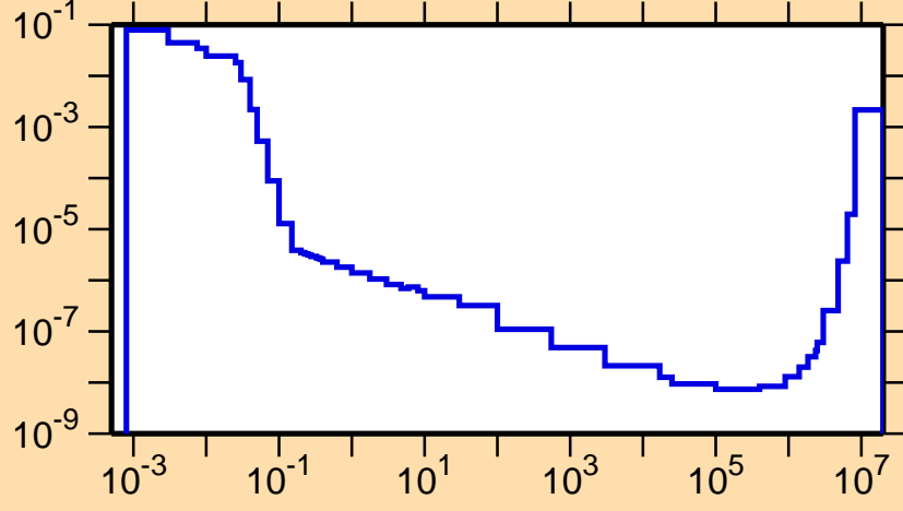
\sigma vs. E for ^{231}\text{Pu}(n,\alpha)
