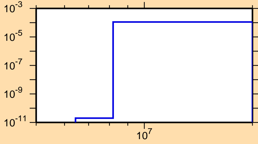
\sigma vs. E for ^{231}\text{Pu}(n,np)
