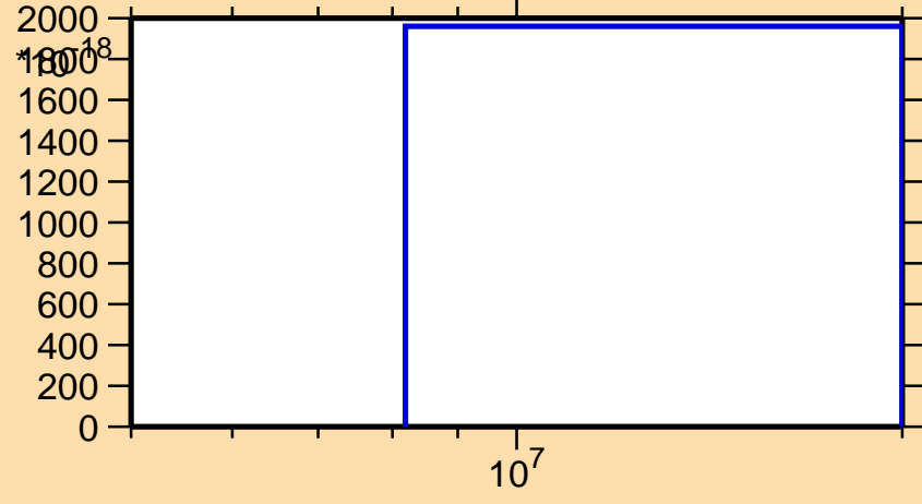
\sigma vs. E for ^{231}\text{Pu}(n,pd)
