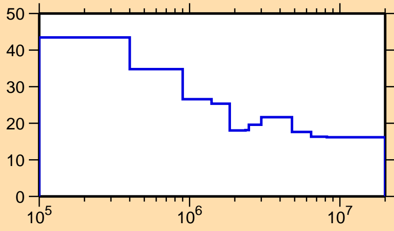
\Delta\sigma/\sigma vs. E for ^{231}\text{Pu}(n,\text{nonel.})
