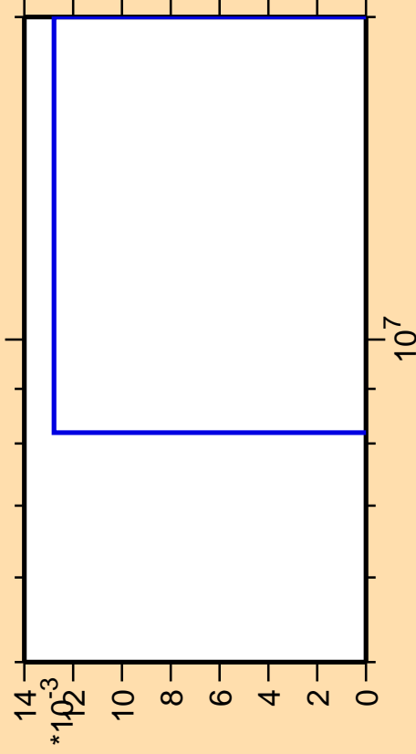
\Delta\sigma/\sigma vs. E for ^{231}\text{Pu}(n,pd)
