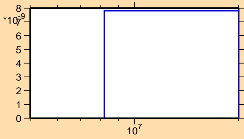
\sigma vs. E for ^{231}\text{Pu}(n,2n\alpha)
