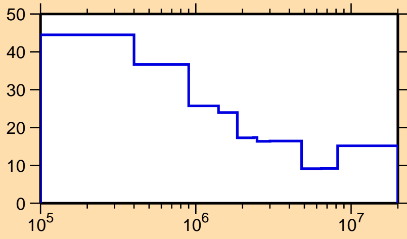
\Delta\sigma/\sigma vs. E for ^{231}\text{Pu}(n, f)
