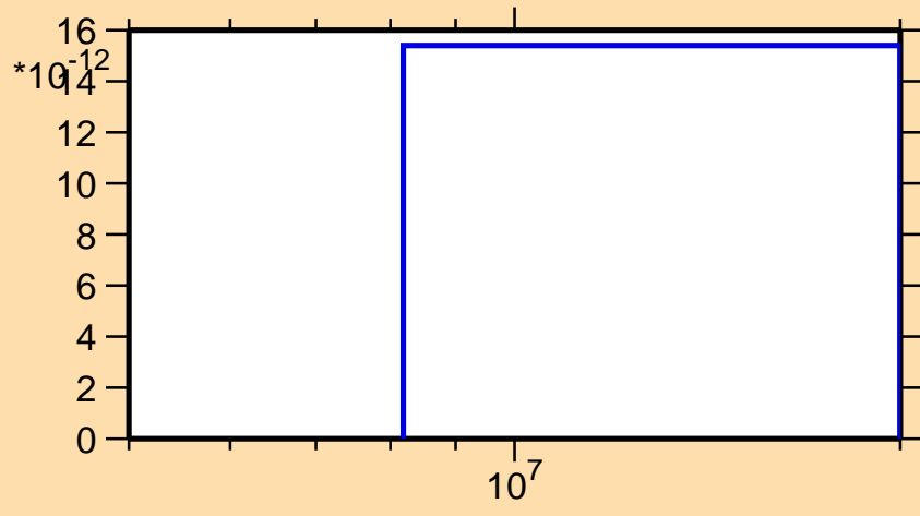
\sigma vs. E for ^{231}\text{Pu}(n,p\alpha)
