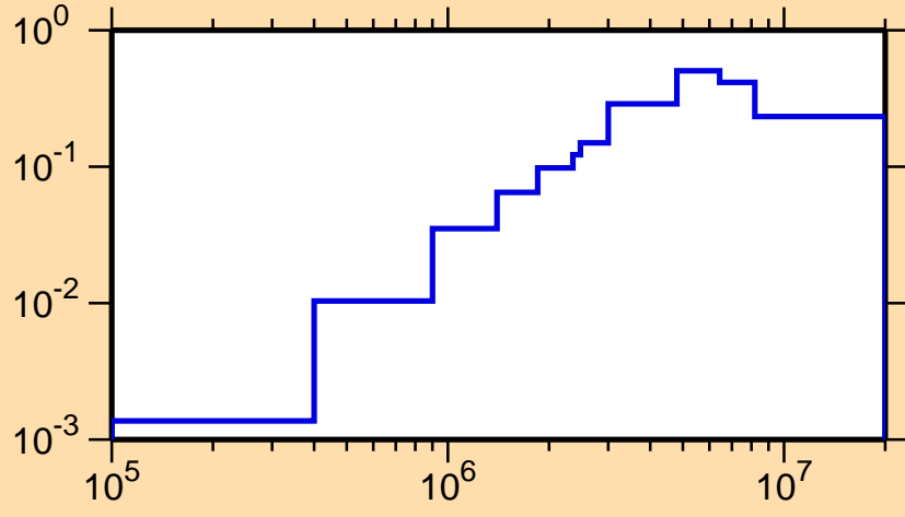
\sigma vs. E for ^{231}\text{Pu}(n,n\text{cont.})
