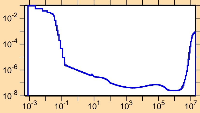
\sigma vs. E for ^{233}\text{Pu}(n,\alpha)
