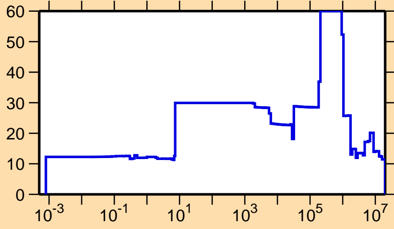
\Delta\sigma/\sigma vs. E for ^{233}\text{Pu}(n,el.)
