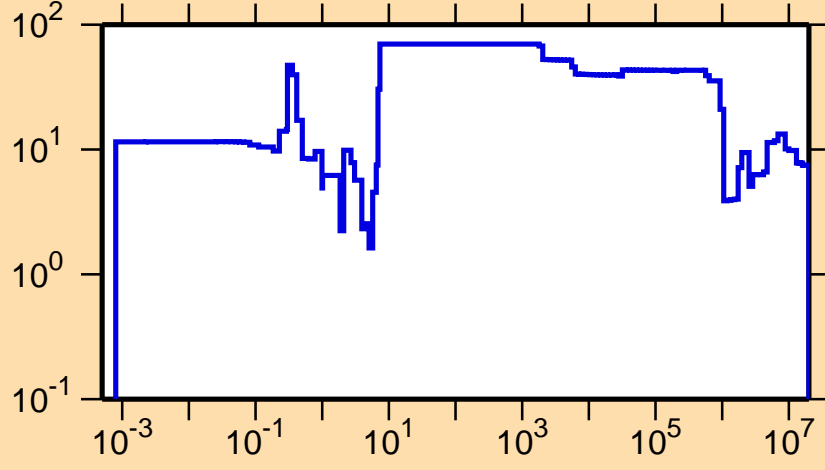
\Delta\sigma/\sigma vs. E for ^{233}\text{Pu}(n,tot.)
