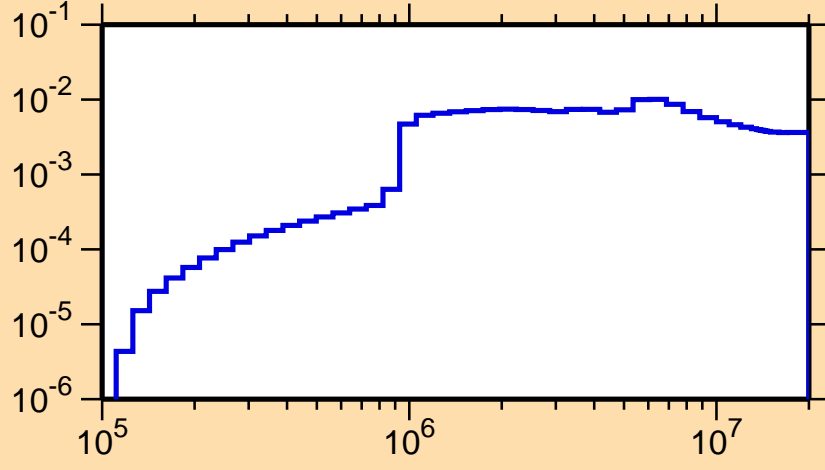
\sigma vs. E for ^{233}\text{Pu}(n,n\text{cont.})
