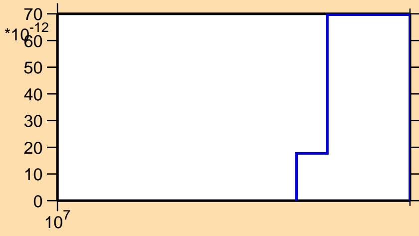
\sigma vs. E for ^{233}\text{Pu}(n,p\alpha)
