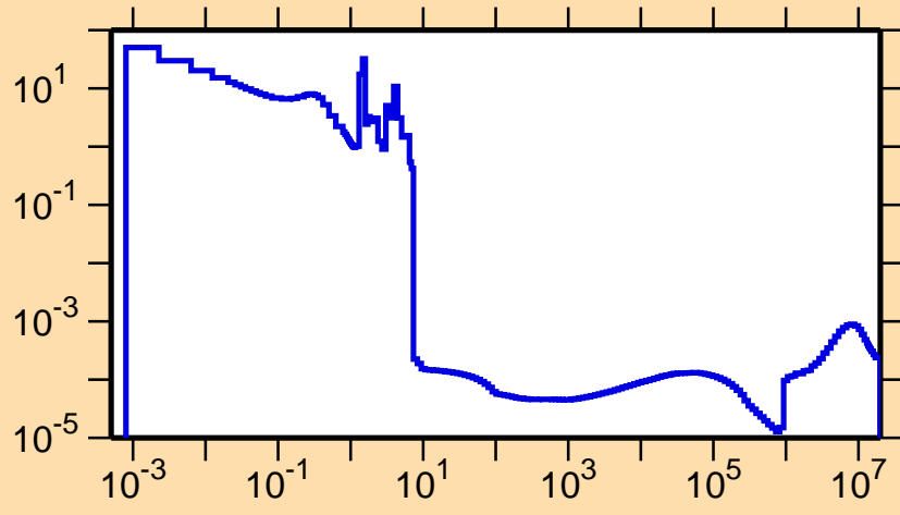
\sigma vs. E for ^{233}\text{Pu}(n,\gamma)
