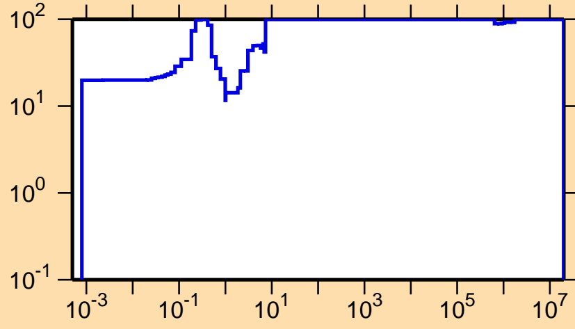
\Delta\sigma/\sigma vs. E for ^{233}\text{Pu}(n,\gamma)
