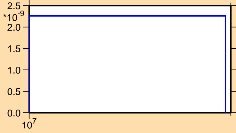
\sigma vs. E for ^{233}\text{Pu}(n,\text{He}3)
