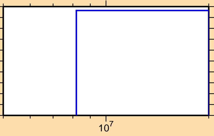
\sigma vs. E for ^{233}\text{Pu}(n,nt)
