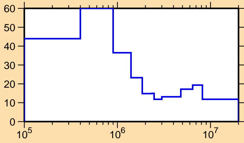
\Delta\sigma/\sigma vs. E for ^{233}\text{Pu}(n, el.)
