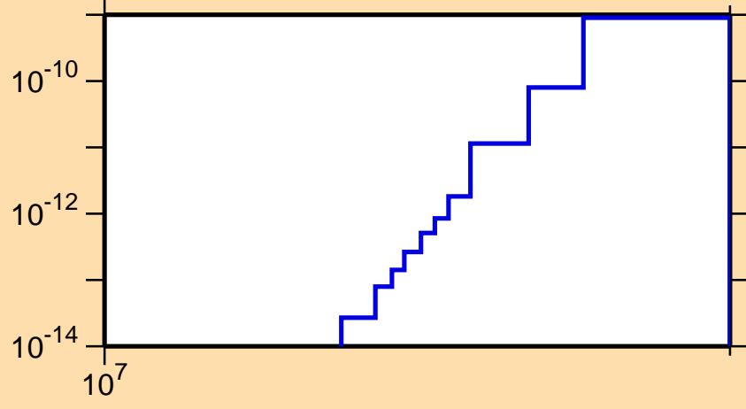
\sigma vs. E for ^{235}\text{Pu}(n,\text{He3})
