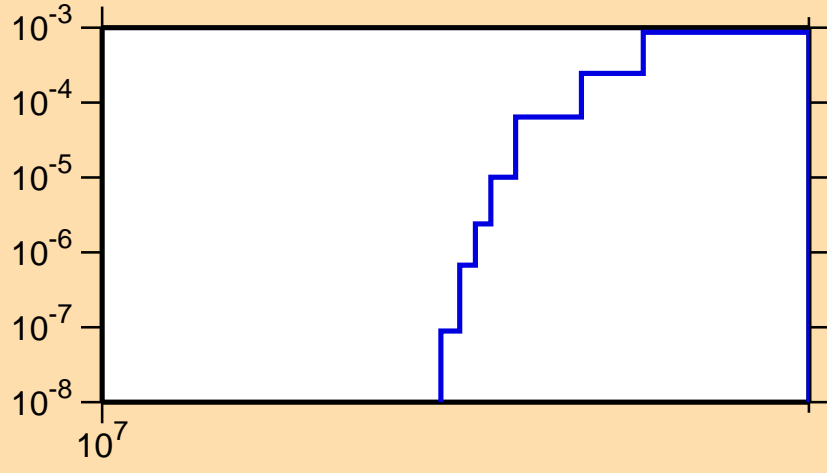
\sigma vs. E for ^{235}\text{Pu}(n,3n)
