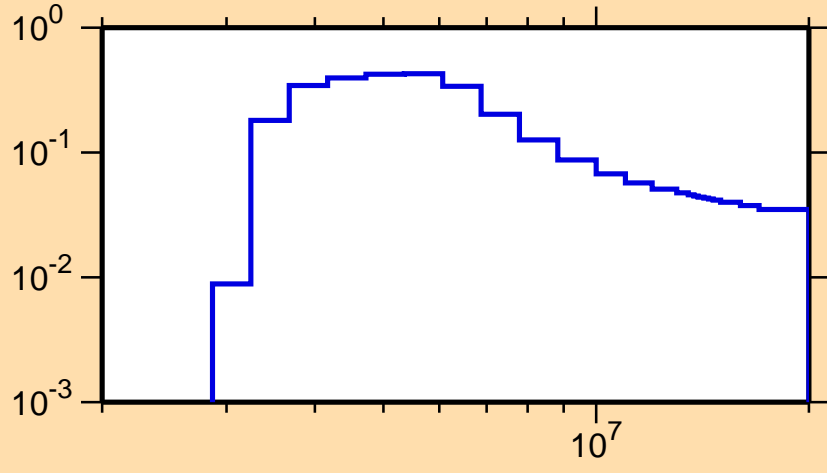
\sigma vs. E for ^{235}\text{Pu}(n,n\text{cont.})
