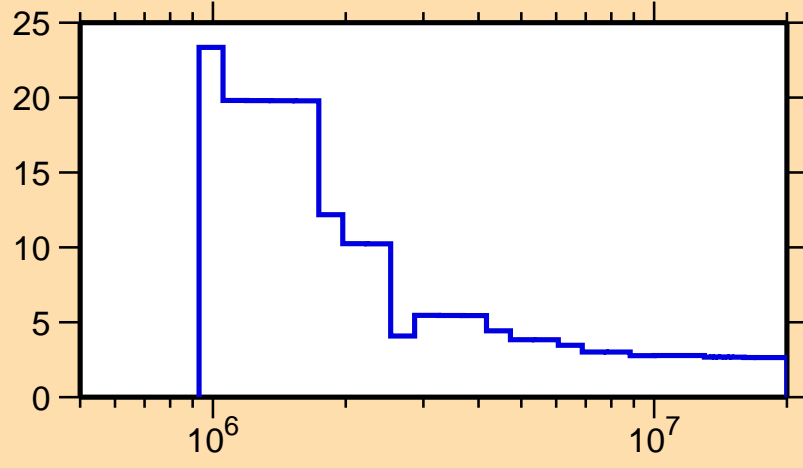
\Delta\sigma/\sigma vs. E for ^{235}\text{Pu}(n,\text{nonel.})
