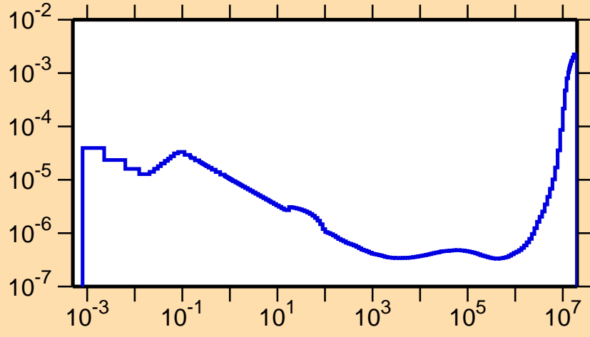
\sigma vs. E for ^{235}\text{Pu}(n,\alpha)
