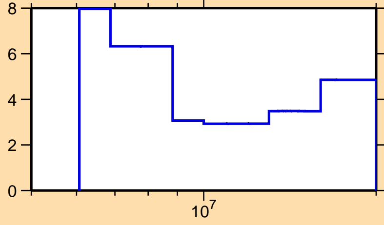
\Delta\sigma/\sigma vs. E for ^{235}\text{Pu}(n,\text{tot.})
