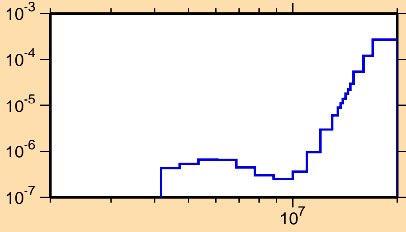
\sigma vs. E for ^{235}\text{Pu}(n,n\alpha)
