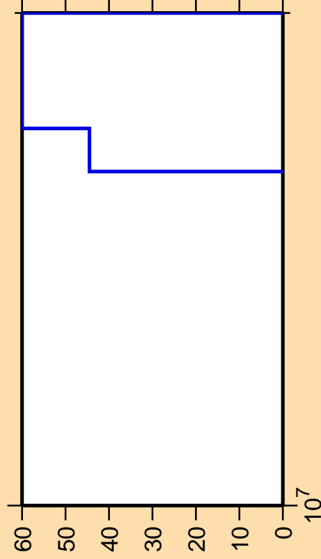
\Delta\sigma/\sigma vs. E for ^{235}\text{Pu}(n,p\alpha)
