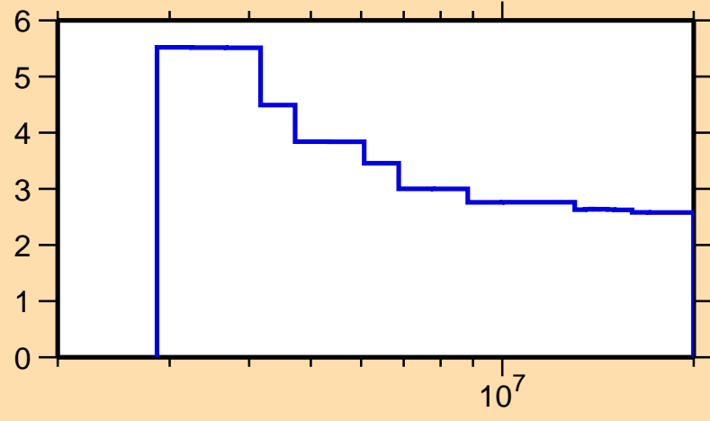
\Delta\sigma/\sigma vs. E for ^{235}\text{Pu}(n, f)
