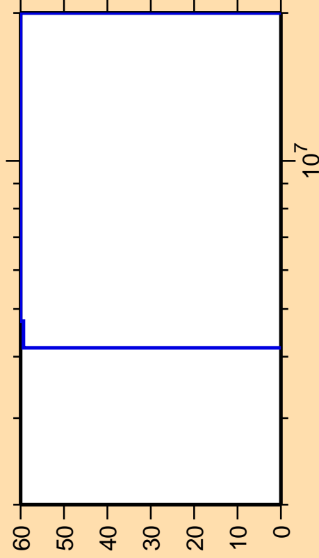
\Delta\sigma/\sigma vs. E for ^{235}\text{Pu}(n,n\alpha)
