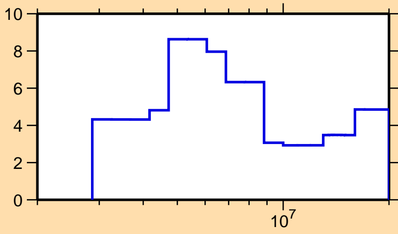
\Delta\sigma/\sigma vs. E for ^{235}\text{Pu}(n,\text{tot.})
