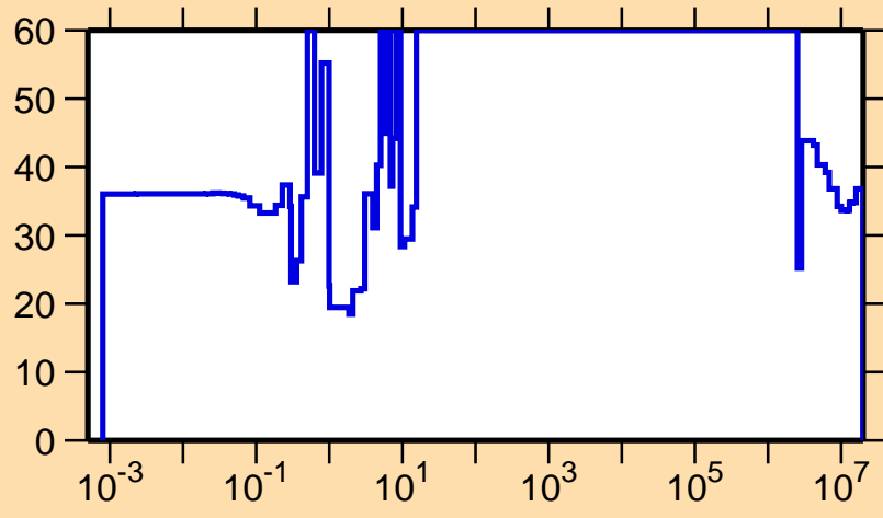
\Delta\sigma/\sigma vs. E for ^{235}\text{Pu}(n,\gamma)
