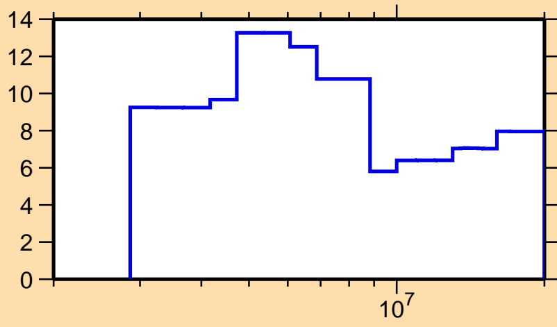
\Delta\sigma/\sigma vs. E for ^{235}\text{Pu}(n,\text{el.})
