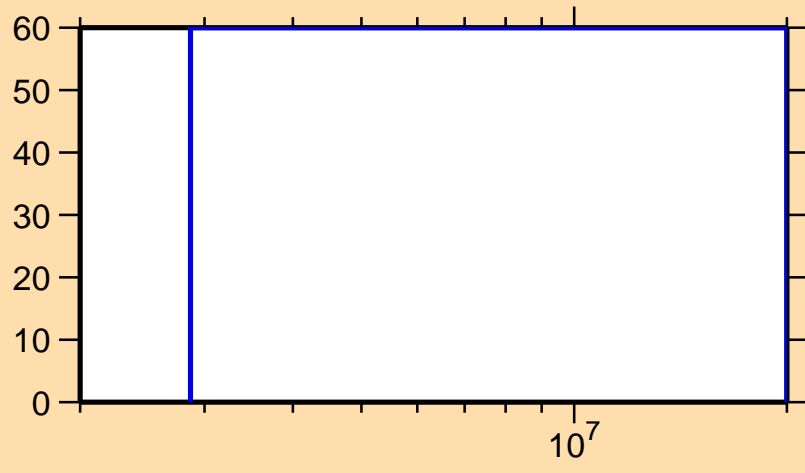
\Delta\sigma/\sigma vs. E for ^{235}\text{Pu}(n,\text{inel.})
