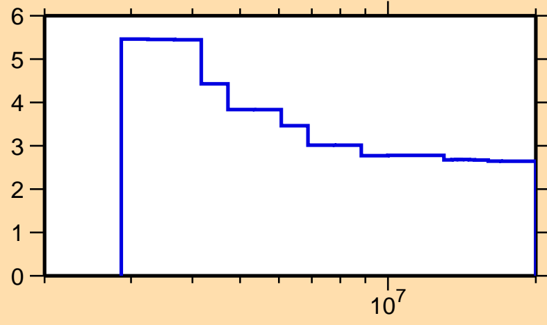
\Delta\sigma/\sigma vs. E for ^{235}\text{Pu}(n,\text{nonel.})
